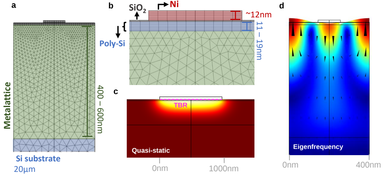
Figure 4.8: Full sample finite element model: (a) Geometry and mesh used in the eigenfrequency simulations of one period of the L = 100 nm, P = 400 nm nickel grating. (b) Zoomed-in geometry and mesh showing the nickel structure, silicon overlayer and thin native oxide layer. The native oxide layer is only included in the eigenfrequency simulations. (c) Simulated temperature profile for a quasi-static thermal simulation some time after the heat pulse given by Eq. 4.16 is injected into the nickel structure. The pink line represents the thermal boundary resistance between the nickel and silicon. (d) Simulated displacement profile from an eigenfrequency calculation showing the mode identified by the SAW-likeness analysis. Figure panel (d) adapted from [68].
