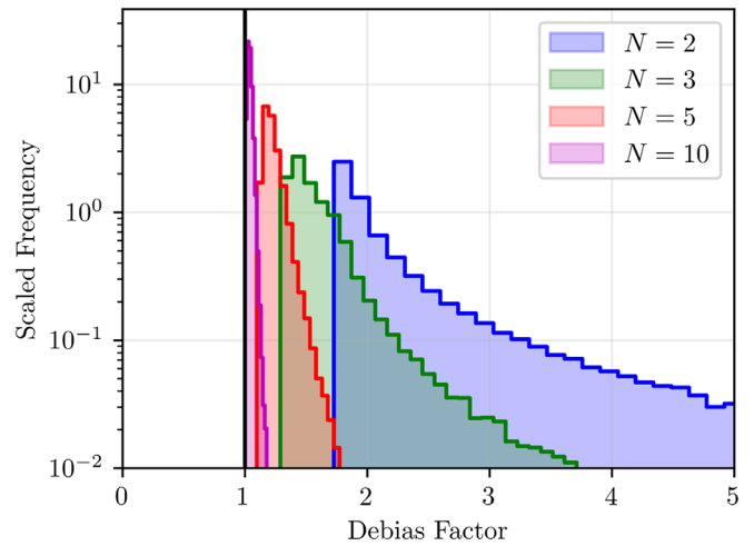
Figure 19. Debias factor associated with M = 10 total points apportioned randomly among N = 2, 3, 5, and 10 sets of replicas.
