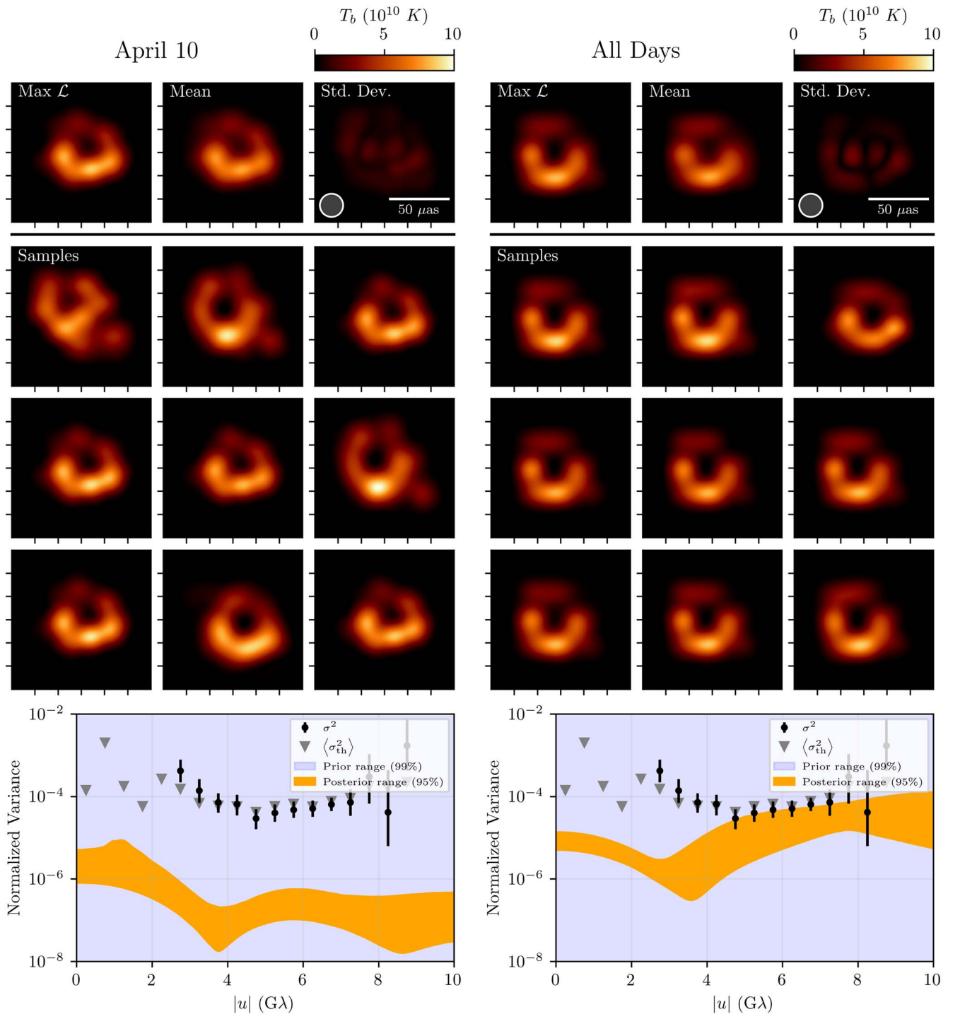
Figure 15. Reconstructed images (top) and noise posteriors (bottom) for the EHT observations of M87 * on a single day (2017 April 10; left) and combined across all days (2017 April 5, 6, 10, and 11; right). The top row shows maximum likelihood (left), posterior average (middle), and standard deviation (right) images, with nine additional random draws from the posterior shown below. To recover physical brightness units, all images have been renormalized by a common factor so that the total flux of the mean image matches the mean of the light curve. In the bottom panels, the reconstructed noise posterior (orange) is shown in comparison to the allowed noise models permitted by the assumed priors (blue, covering the entire range) and typical thermal noise estimates (gray triangles). For reference, the data-driven nonparametric variance estimates from Figure 14, constructed from the full 2017 EHT M87 * campaign, are reproduced (black points).
