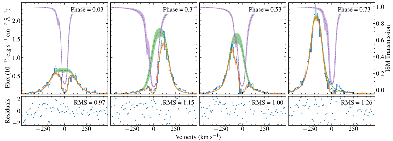
Figure 3. Fits to the Ly \alpha emission line in all four G140M spectra, ordered by orbital phase. The observed spectrum is shown in blue with error bars on every third point. The intrinsic Ly \alpha profile is shown in green and the ISM transmission in purple, both of which are convolved to the instrumental resolution. The product of these profiles is the final fit to the data (orange). Shaded areas behind each profile show the 1\sigma uncertainties of the model fits. The bottom panel shows the residuals, calculated as (data – model)/data uncertainty.
