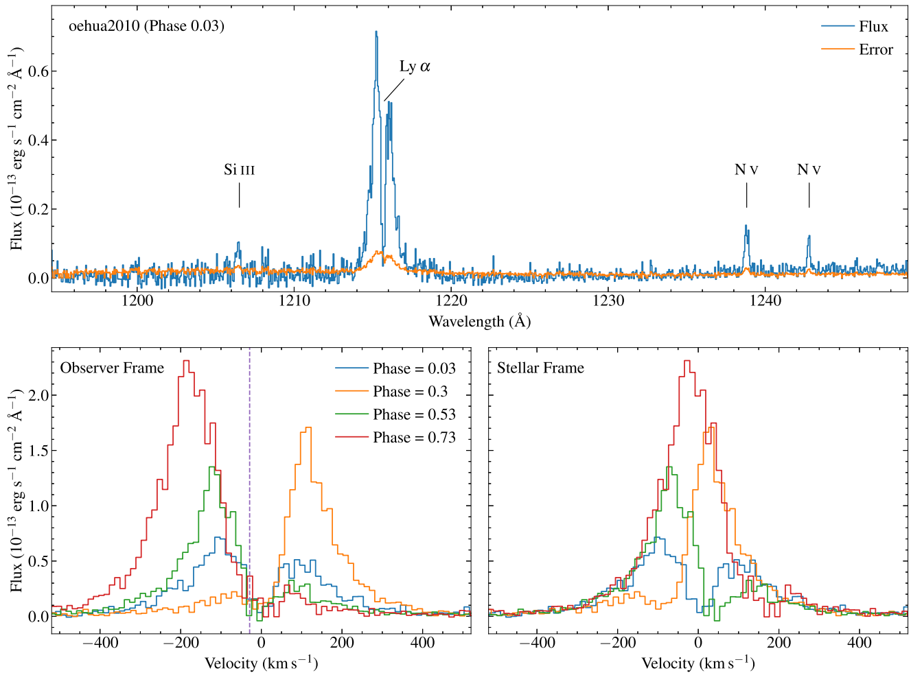
Figure 2. Top panel: example STIS G140M spectrum of EG UMa (data set OEHUA2010) with major emission features marked. Note the increased scatter noise at wavelengths \lesssim 1214 Å due to the FUV glow. Bottom panels: the Ly \alpha emission line in all four spectra, in the observer rest frame (left) and velocity-shifted to the M dwarf rest frame (right). The dashed purple line in the left panel shows the center-of-mass radial velocity of the binary system.
