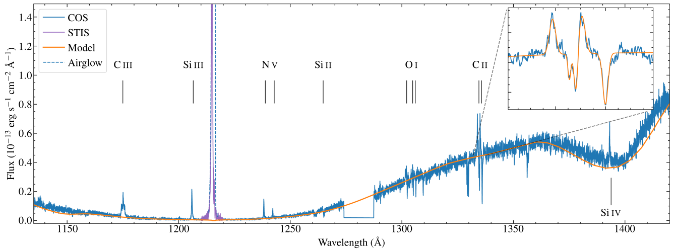
Figure 1. Far-ultraviolet spectrum of EG UMa. The COS spectrum is shown in blue, with a dashed line indicating the region affected by geocoronal Ly \alpha airglow. Prominent emission (from the M dwarf atmosphere) and absorption (stellar wind accretion onto the white dwarf) features are labeled. The white dwarf model spectrum is shown in orange. The STIS spectrum shows the highest-velocity and mostly unobscured Ly \alpha line at phase 0.73, which exceeds the axis limit by factor \approx 2 . The inset shows the region around the C II 1335 Å lines, simultaneously fit with an ASTROPY model to measure the instantaneous radial velocity of the M dwarf (emission features), ISM (weak absorption features), and the white dwarf (strong absorption features).
