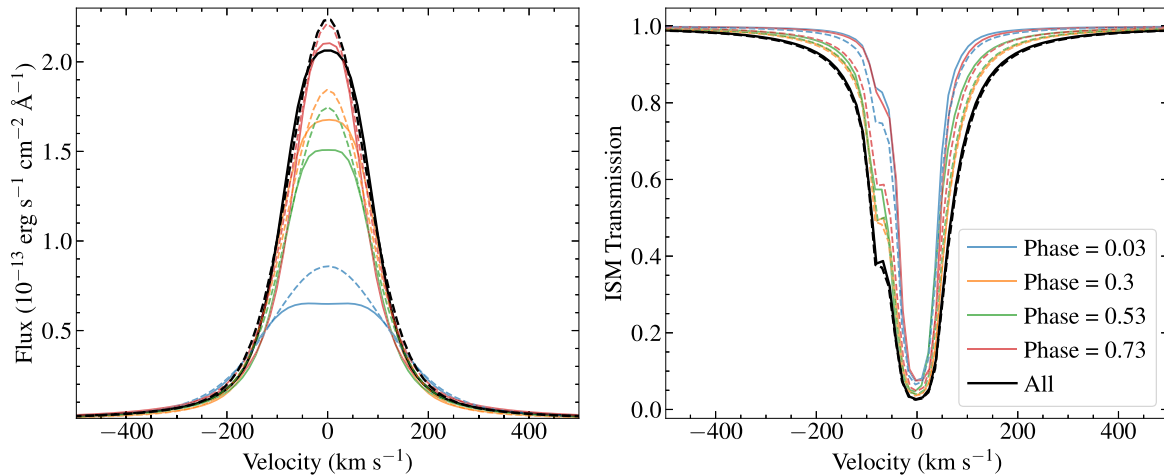
Figure 6. Left: intrinsic Ly \alpha line profiles reconstructed from the individual spectra, along with the simultaneous fit to all four, velocity-shifted to the rest frame. Results from fits not including self-reversal are shown as dashed lines. Right: the same for the ISM profile. In both panels, the profiles have been convolved with the STIS G140M line-spread function.
