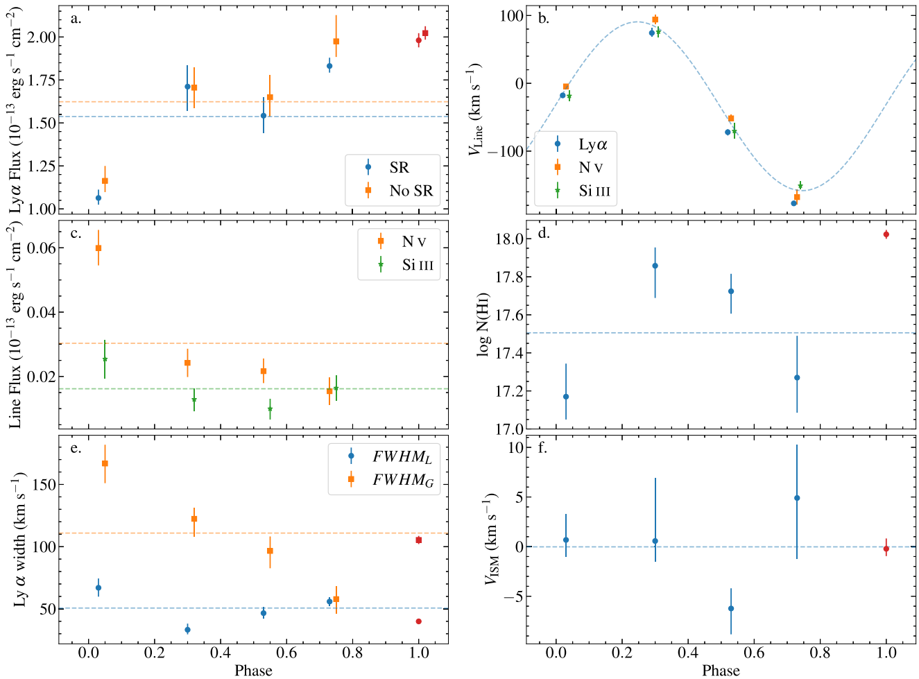
Figure 5. Summary of the reconstruction results. (a) The intrinsic flux of the best-fit Ly \alpha line for each spectrum, comparing fits with and without self-reversal (SR). (b) The radial velocities of the emission lines. (c) The integrated fluxes of the Si III and N V emission lines, where N V is the combined flux of the doublet. (d) The ISM hydrogen column density. (e) The Voigt widths of the best-fit Ly \alpha line. (f) The radial velocity of the ISM. The dashed lines show the mean value of each quantity, except for panel (b), where the radial velocity curve of the M dwarf is shown. In all panels, the red points at phase = 1.0 show the results for the simultaneous fit to all four spectra, which are not included in the means. All results are for fits including self-reversal except where noted in panel (a). Small phase offsets have been applied where necessary to avoid overlapping points.
