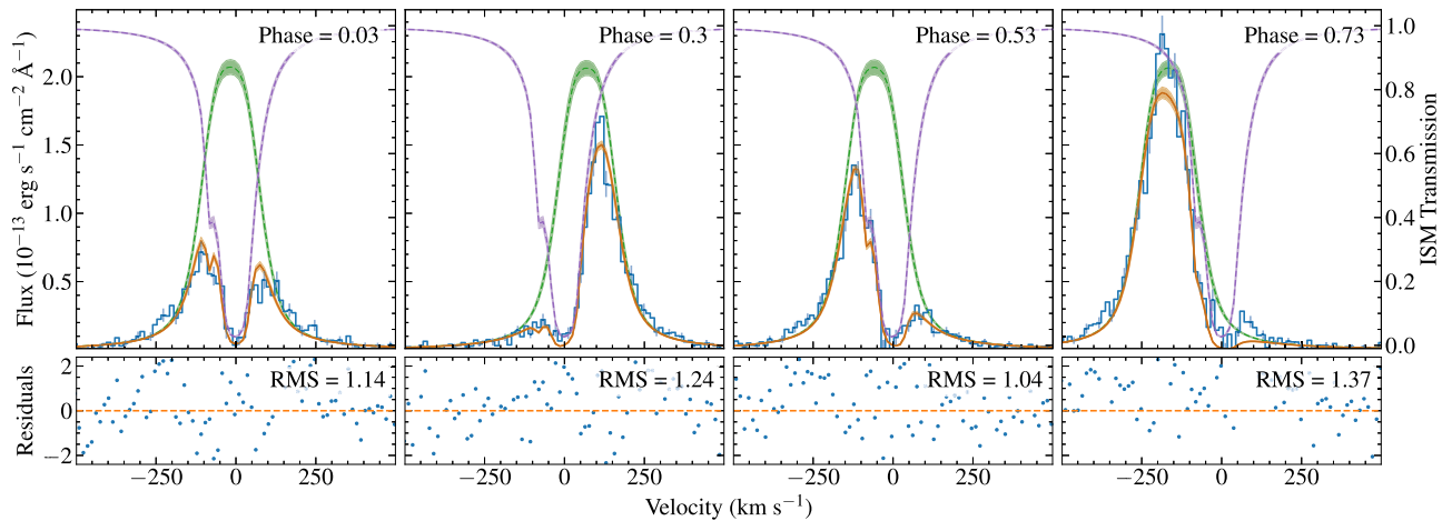
Figure 4. As Figure 3, but fitting all four spectra simultaneously with only the radial velocity allowed to vary between reconstructions.
