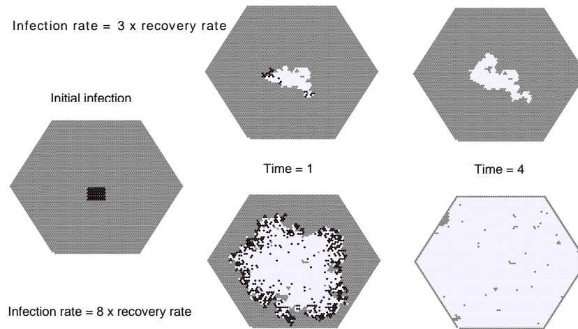
Figure 10. A susceptible–infectious–recovered (SIR) model built with CellLab-CTS. This example compares runs with two different infection rates (top and bottom rows, respectively). Gray is susceptible, black is infectious, and white is recovered. One time unit is one average recovery time. This example model uses the HexCTS subclass (non-oriented model with hexagonal cells).
