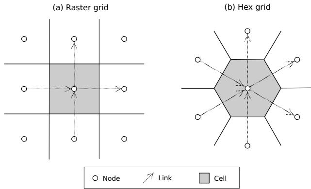
Figure 3. Schematic illustration of CellLab-CTS grid types and geometric primitives. (a) Regular (raster). (b) Trigonal lattice with hexagonal cells. Note that standard link orientation is within the x \geq y half plane; in other words, the angle of a link, \theta , with respect to the positive x axis is always -45^\circ \leq \theta \leq 135^\circ .
