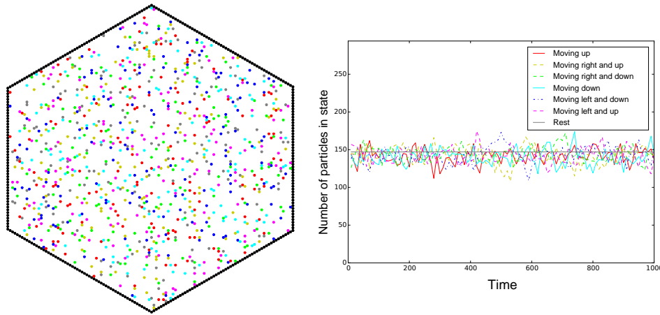
Figure 12. Example of a CTS lattice gas model. Left: particles undergoing random (brownian) motion in a vessel. Color codes: white is empty, black is wall, and gray is resting; others moving in the directions indicated in inset legend. Right: number of particles in each movement direction versus time, illustrating the conservation of average momentum.
