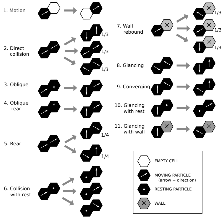
Figure 11. Motion and collision rules for a pairwise CTS lattice gas model. For states that have multiple transitions, the transition rate for each is reduced from unity to the fraction shown. Reduction to a one-fourth rate (instead of one-half) for rear collisions accounts for the possibility that the lead particle is faster (so no collision occurs).
