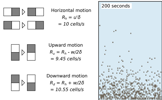
Figure 2. Turbulent suspension model with grains (1 mm tea leaves) that are 0.2% denser than the surrounding fluid. Left: illustration of cell-pair transitions representing motion in the four directions. Grain settling velocity of 0.0011 \text{ m s}^{-1} imparts asymmetry to the transition probabilities.
