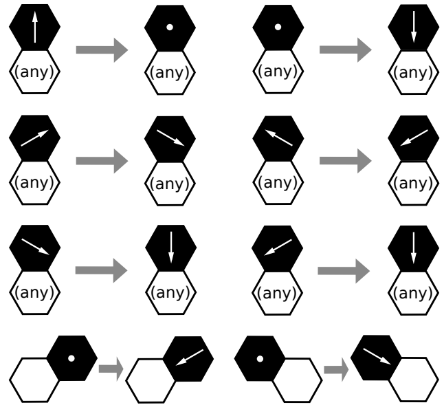
Figure 14. Gravity rules for lattice-grain model. Each transition has a rate g . The bottom two transitions represent angle-of-repose behavior. This example uses the OrientedHexCTS subclass.
