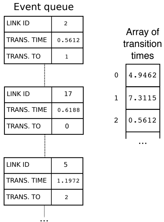
Figure 6. Illustration of the event queue and the transition-time array ( next_update ). Each event object contains the ID number of the link, the time at which the next transition is scheduled to occur, and the link-state code for the transition (that is, the code for the new cell pair after transition occurs). Left: events are stored in a heap that is sorted by transition time, soonest on top. Right: the transition-time array, which is simply an ordered array, indexed by link ID, containing the time of the next scheduled transition at the corresponding link. If the transition time for an event object does not match the corresponding entry in the transition-time array, it means that the originally scheduled transition has been nullified by other transitions and is no longer valid (see text).
