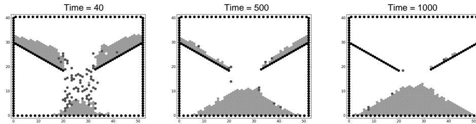
Figure 15. Three snapshots from a lattice-grain simulation showing the emptying of a silo. Color codes: white is empty, black is wall, light gray is resting grain, and dark gray is moving grain.
