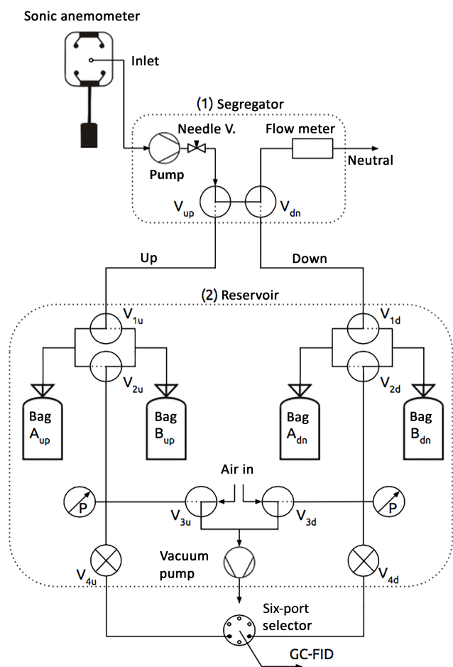
Figure 2. The relaxed eddy accumulation (REA) system is comprised of (1) a segregator subsystem and (2) a reservoir subsystem. Sample valves are indicated by V, with updraft (up) and downdraft (dn) air sampling valves and bag reservoirs shown.
