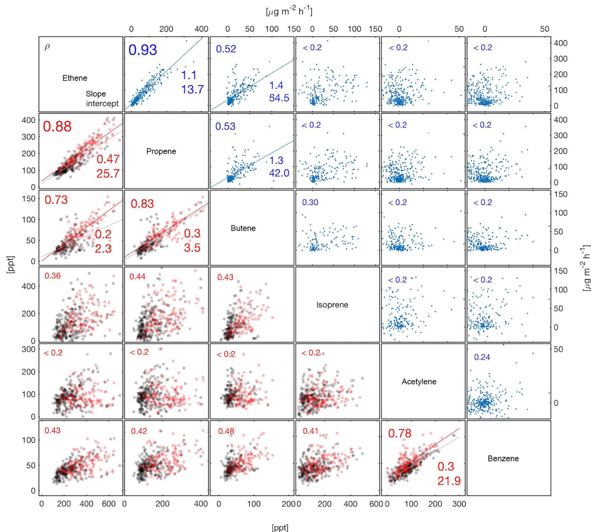
Figure 7. Correlation matrix of light alkene, isoprene, acetylene and benzene fluxes (blue), daytime concentrations (red) and nighttime concentrations (black). Numbers denote the Pearson correlation coefficient ( \rho , top left) and the slope and intercept (bottom right numbers) for the linear fits in plots where \rho > 0.5 . Negative fluxes for the light alkenes (1.3 to 2.3 % of the light alkene fluxes) are excluded from the plot and the regression statistics; positive fluxes < LDL are not excluded.
