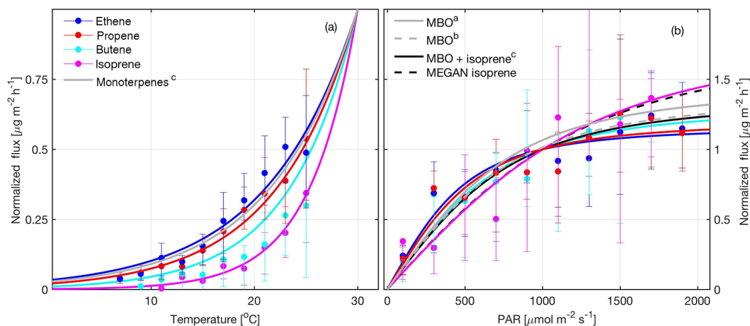
Figure 9. Parameterized response curves (solid lines) of alkene fluxes with 10th–90th percentile (error bars) for (a) the light-independent fraction (LIDF) temperature response (Eq. 5) bin-averaged into 2 °C classes and (b) the PAR-dependent response (Eq. 4) bin-averaged into 200 \mu\text{mol m}^{-2} \text{s}^{-1} classes. Response curves are normalized to a flux of 1 at (a) a reference temperature of 30 °C and (b) a reference PAR of 1000 \mu\text{mol m}^{-2} \text{s}^{-1} . The light-dependent fraction (LDF) temperature response (Eq. 6) curve fit is shown in the Supplement (Fig. S5). The response curves in gray and black are for other BVOCs as cited in Tables 2 and 3: b Harley et al. (1998); c Schade and Goldstein (2001); d Kaser et al. (2013a).
