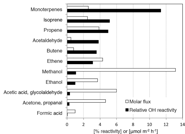
Figure 8. Daytime averaged molar flux and relative OH reactivity for the major known BVOCs emitted at Manitou Experimental Forest. MBO (not shown) contributes 21\ \mu\text{mol m}^{-2}\ \text{h}^{-1} and 65% of the OH reactivity.
