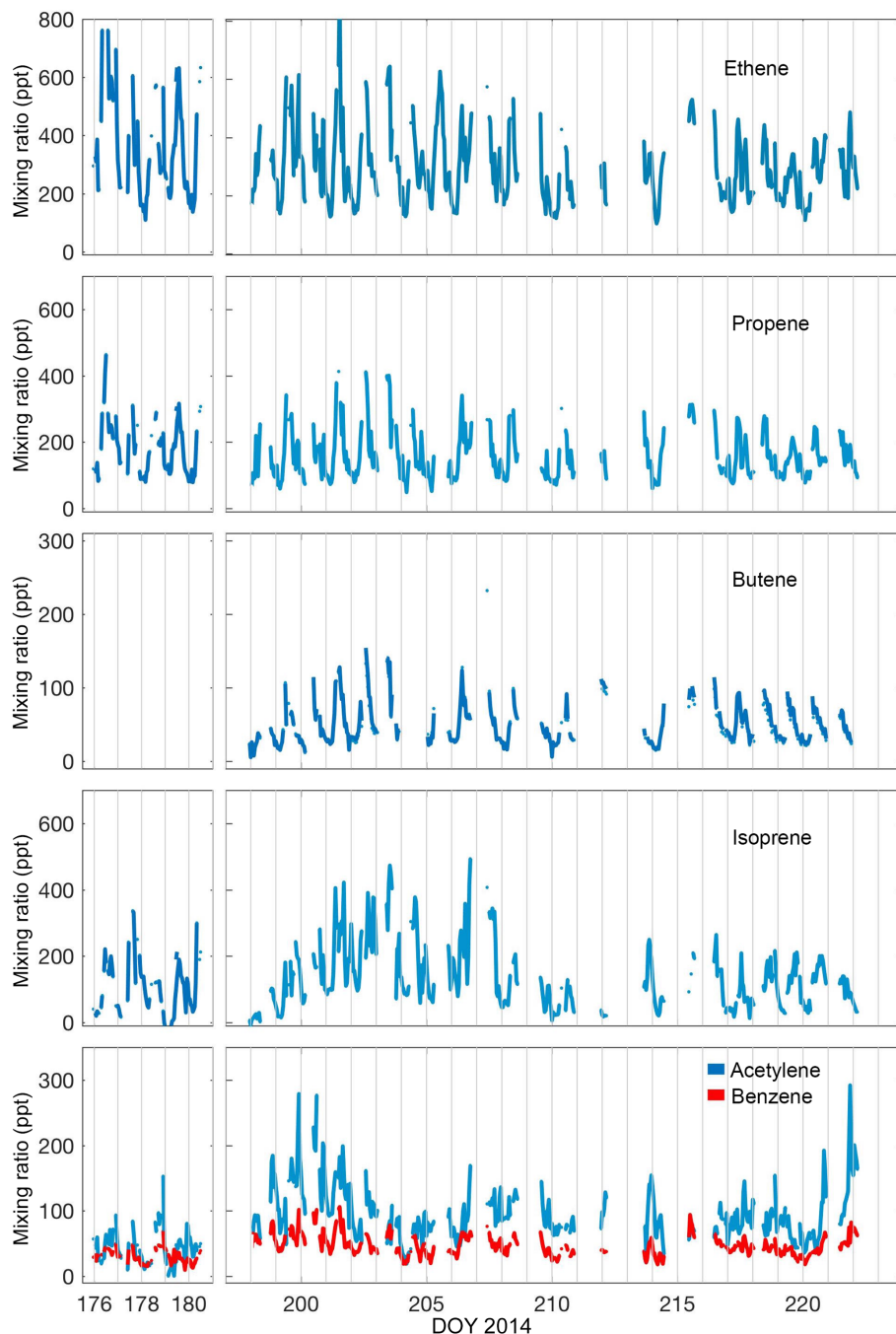
Figure 4. Hourly averaged ambient concentrations of alkenes, acetylene and benzene at Manitou Forest. Periods of missing data are due to instrumental maintenance or incomplete chromatography.
