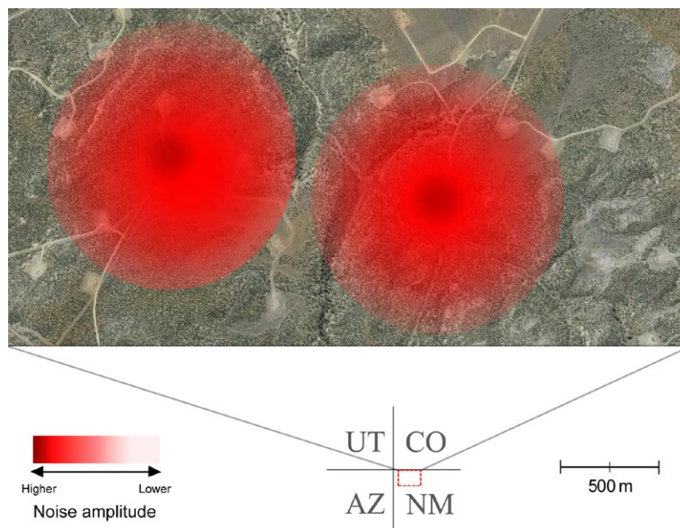
Fig. 1. Rattlesnake Canyon Habitat Management Area (red outline) is located in northwestern New Mexico, near the Colorado border in San Juan County. Noise increases in intensity near the compressors and is represented by red spheres that extend 650 m from the point source.
