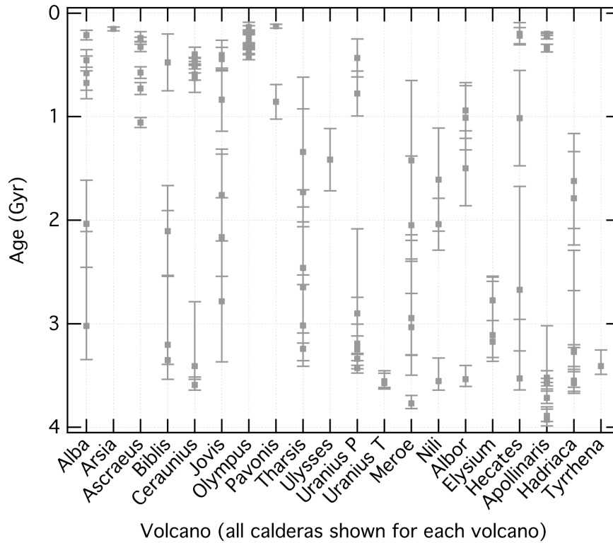
Figure 57: Timeline illustrating the ages discussed in the text and Table 9 for every volcano in this study. Split ages for a single caldera are included in this figure, even though several are likely due to resurfacing processes (e.g., Ceraunius Tholus for calderas 3 and 4).
