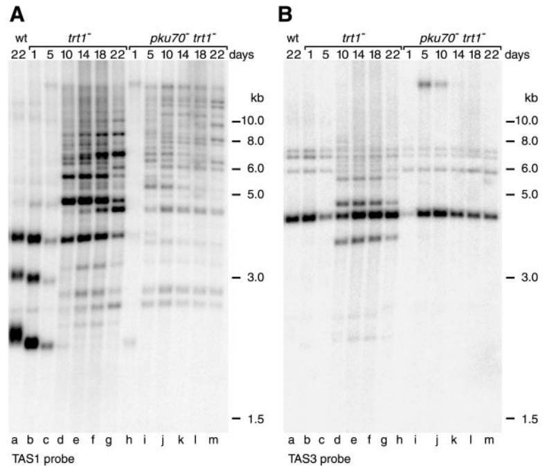
Figure 5. Dynamic rearrangements of TAS in survivors of senescence. (A) Genomic DNA ( 15 \mu\text{g} ) was prepared from trt1 - and pku70 - trt1 - cultures on the indicated days, digested with Nsi I, and fractionated on agarose gels. DNA was transferred onto a nylon membrane and hybridized to a 32 P-labeled TAS1 probe. Size markers are as in Figure 2. (B) The blot shown in A was stripped as described in MATERIALS AND METHODS and hybridized to a TAS3 probe.
