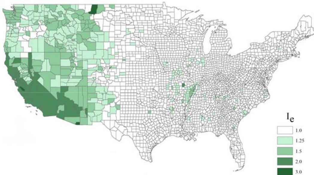
Figure 16: Maximum strength and stiffness factor I_e to exceed 2015 IBC and IRC seismic design requirements where the incremental benefit remains cost effective.
