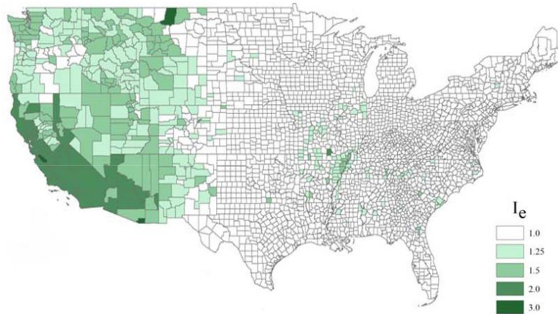
Figure 2-15 : Maximum strength and stiffness factor I_e to exceed 2015 IBC and IRC seismic design requirements where the incremental benefit remains cost effective.
