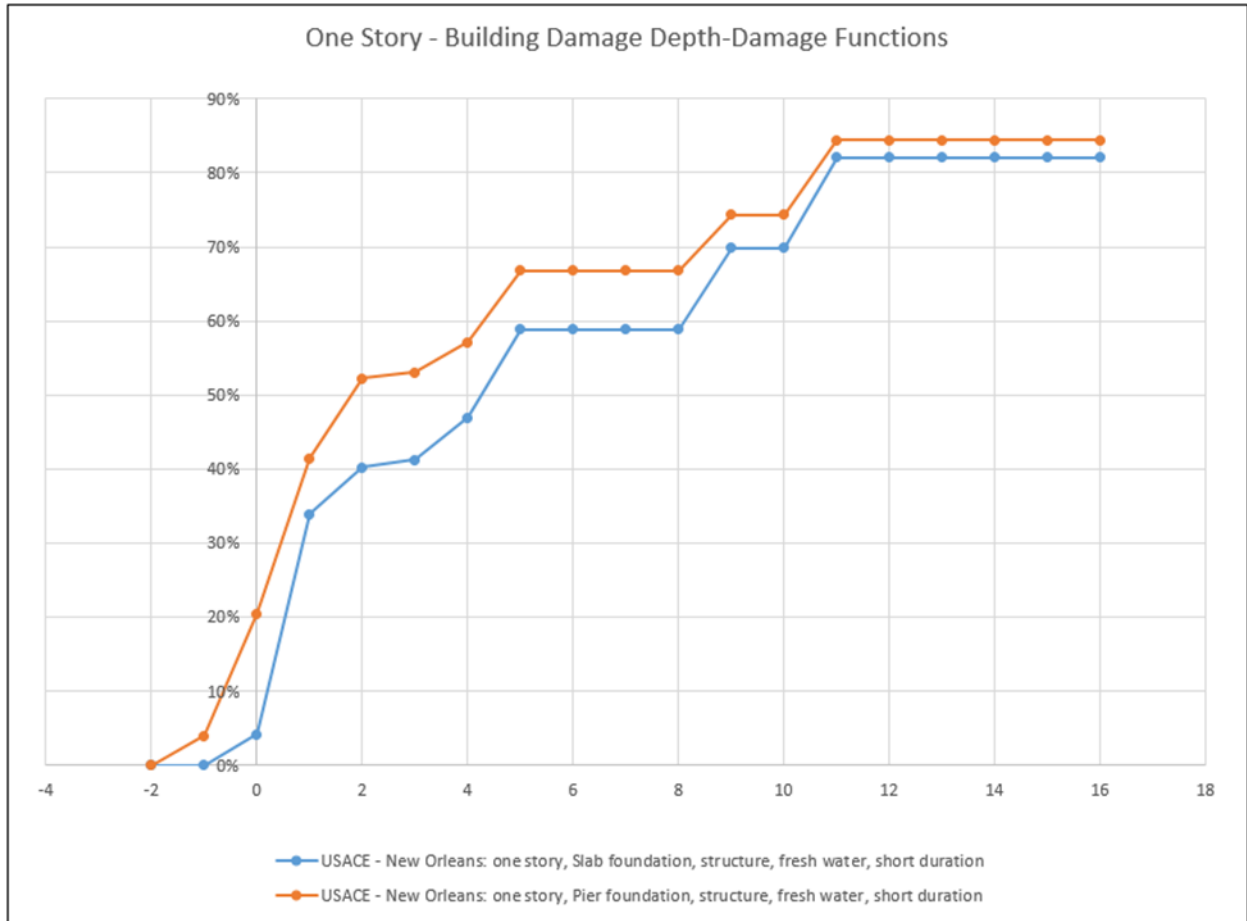
Figure 5-12: Depth-damage functions for one-story houses.
