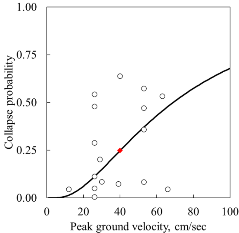
Figure 4-4: Fragility function and collapse data for manufactured housing in the epicentral region of the 1989 Loma Prieta earthquake.
