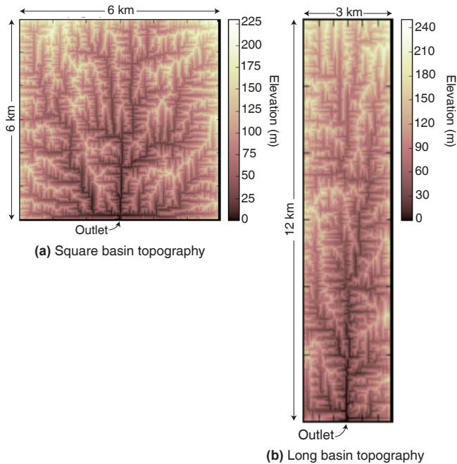
Figure 9. Two test basins evolved using the Landlab FlowRouter and StreamPowerEroder components (not described here; see Hobbey et al., 2017), generating a network using D4 flow routing and erosion methods. Each grid was evolved from an initial random topography to steady state, where uplift rate is matched by incision rate. Both basins have the same drainage area ( 36 \text{ km}^2 ) at the watershed outlet but different dimensions: panel (a) has 200 rows \times 200 columns, and panel (b) has 400 rows \times 100 columns. Both have a grid resolution ( \Delta x ) of 30 m. Note the perpendicular junctions are due to the D4 flow routing scheme.
