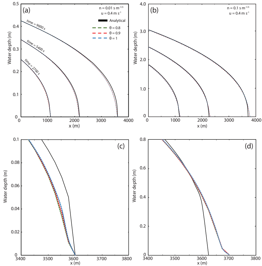
Figure 7. Sensitivity of the Landlab OverlandFlow component with a changing Manning’s n , compared to the analytical solution. This figure is illustrated in the same manner as Fig. (2) from de Almeida et al. (2012). Water depth was plotted against distance for two combinations of velocity and friction coefficient values. Both panels (a) and (b) show water depths for t = 2700 , 5400 , and 9000 s. Panels (c) and (d) are zoomed-in images of the wave fronts from panels (a) and (b), respectively, at time = 9000 s.
