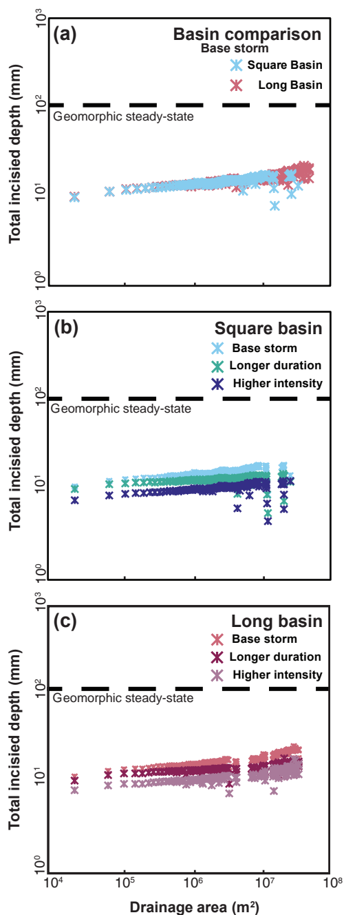
Figure 11. DetachmentLtdErosion output for all storms described in Table 4. Incision depth was taken after 10 years of modeled storms from the OverlandFlow component for all grid locations. The average incision depth was plotted at each drainage area: panel (a) shows incision depth versus drainage area for both the square and long basins after 10 years of the base storm; panel (b) shows total incision results from the square basin for all three precipitation events after 10 years; and panel (c) shows total incision results from the long basin for all three precipitation events after 10 years.
