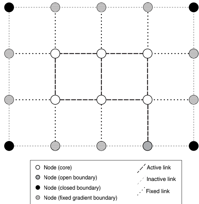
Figure 4. Simple example of Landlab RasterModelGrid, demonstrating both node and link boundary conditions. The OverlandFlow class calculates fluxes at active links, and can update the surrounding fixed links according to these fluxes. No fluxes are calculated at inactive links. Water depth is updated at core and open boundary nodes. No calculations are performed on closed or fixed gradient boundaries. Note that RasterModelGrid cell elements and link directionalities are not illustrated here.
