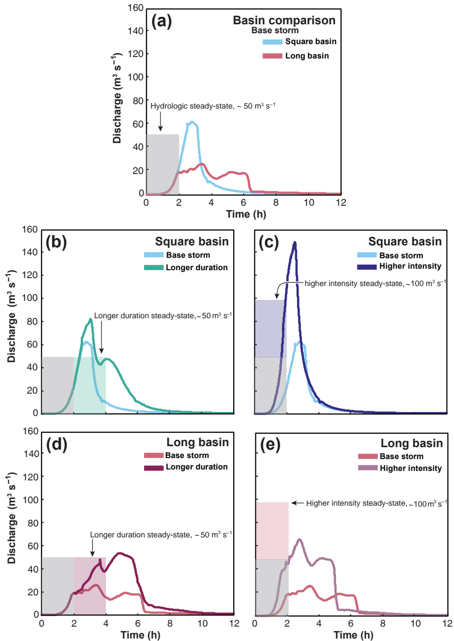
Figure 10. OverlandFlow output for all storms described in Table 4. Hydrographs are taken from the active link upstream of the outlet node. Steady-state discharge is shown for each event, with the gray box representing the base storm in all cases. Panel (a) shows the base storm for both the square basin and the long basin; panel (b) compares outlet hydrographs from the base and longer duration storms in the square basin; panel (c) compares outlet hydrographs from the base and higher intensity storms in the square basin; panel (d) compares outlet hydrographs from the base and longer duration storms in the long basin; panel (e) compares outlet hydrographs from the base and higher intensity storms in the long basin.
