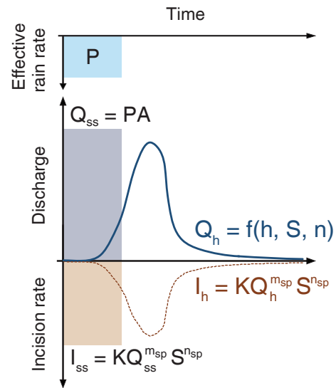
Figure 1. Image illustrating the differences between steady-state and non-steady hydrology and incision at a single point within a watershed. In this schematic, the effective precipitation rate ( P ) is the same for both steady and non-steady cases. During the precipitation event, steady discharge ( Q_{ss} ) and incision rate ( I_{ss} ) are constant, driven by that effective precipitation rate and drainage area ( A ), erodibility ( K ), water surface slope ( S ), and stream power exponents ( m_{sp} , n_{sp} ). In the non-steady case, a wave front begins to propagate and incise, producing time-varying discharge ( Q_h ), calculated using physical parameters such as water depth ( h ), water surface slope ( S ), and Manning's roughness coefficient ( n ). Non-steady incision rate ( I_h ) is calculated using the time-varying discharge, erodibility, and water surface slope. At the end of the precipitation event, Q_{ss} and I_{ss} also end, while non-steady values Q_h and I_h continue until all water has completely exited the system at the outlet.
