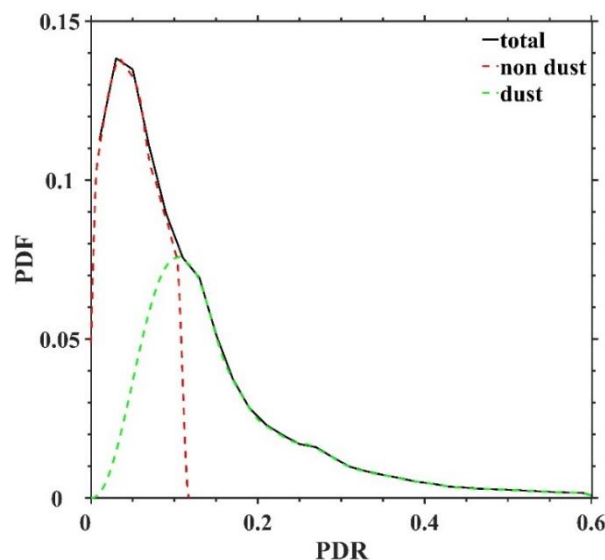
Figure 1. The probability density functions (PDF) of particle depolarization ratio (PDR) for all aerosols observed by MPL from January 2013 to September 2017 at the NSA site. The black line is for all the aerosols derived from MPL observations, while the red and green lines indicate non-dust and dust aerosol modes fitted to the shape of the PDF of all aerosol PDR. A PDR of 0.10 is the cross point of the dust and non-dust aerosol modes.
