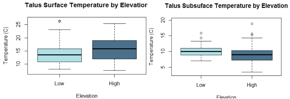
Figures 2a and 2b: Talus sub-surface and surface temperature by elevation.
