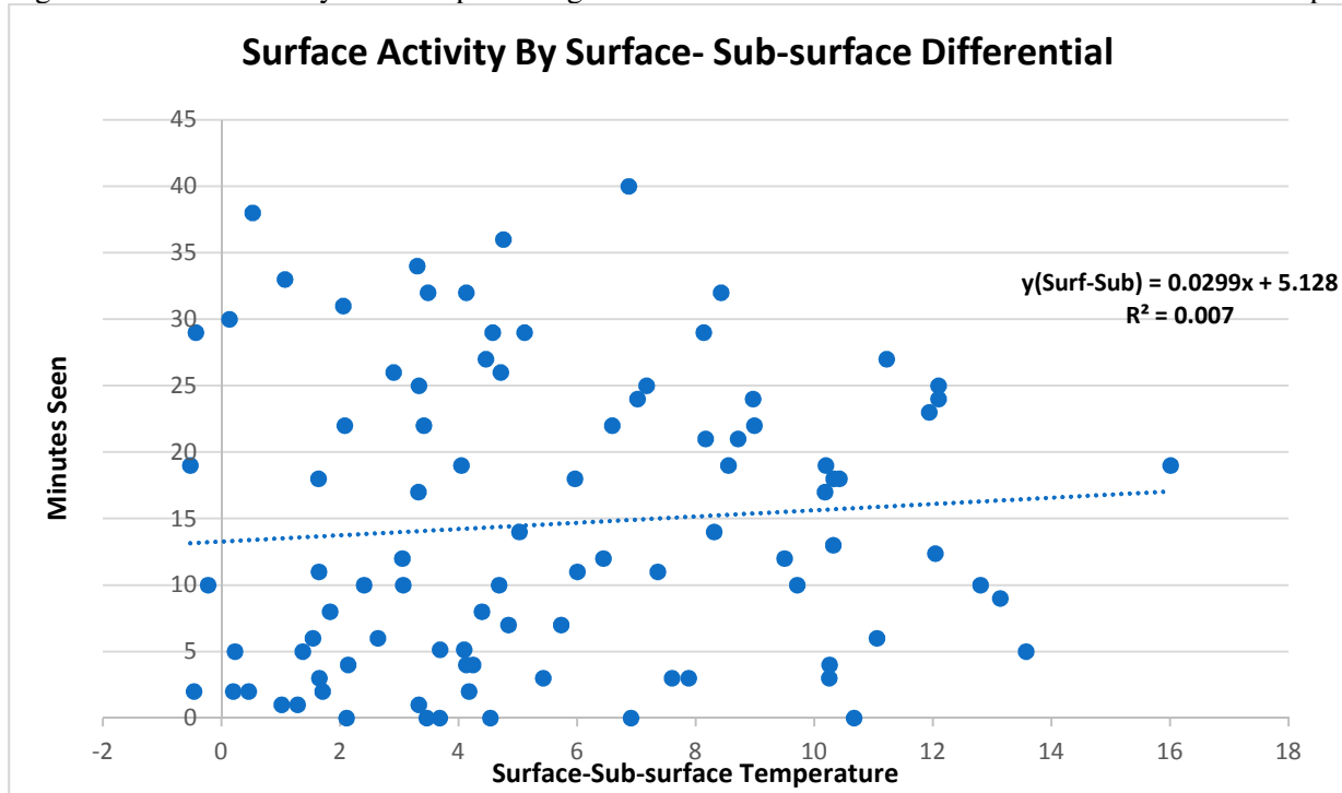
Figure 7: Surface activity-minutes plotted against the difference between surface and sub-surface temperatures.
