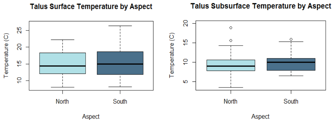
Figures 3a and 3b: Talus surface and sub-surface temperature by aspect.
