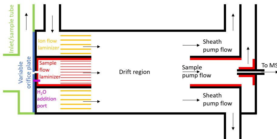
Figure 1. Schematic of the new, coaxial, low-pressure IMR design for CIMS. This is a two-dimensional cross section of the cylindrical IMR along the axis of flow, and it is not to exact scale. Black lines represent stainless steel surfaces, green and blue lines represent PTFE Teflon, and red/yellow lines represent FEP or PFA Teflon. Constant mass flow into the IMR is controlled using a variable orifice. Water vapor can be added through a port in the orifice plate, in order to keep the environmental conditions in the IMR more constant. The sample flow and ion flow are passed through laminizer elements to limit the effects of turbulent diffusion to the IMR walls. Ion–molecule adducts are formed via diffusive mixing in the drift region. The ability to enhance the mixing of ions into the sample flow by applying an electric field between the drift region wall and the exit of the sample flow laminizer was also included (not shown) but led to only modest enhancement and was not used in the measurements presented herein. A mirrored pumping scheme also prevents turbulence and limits the effects of wall interactions. Adducts are sampled through a capillary into the time-of-flight mass spectrometer.
