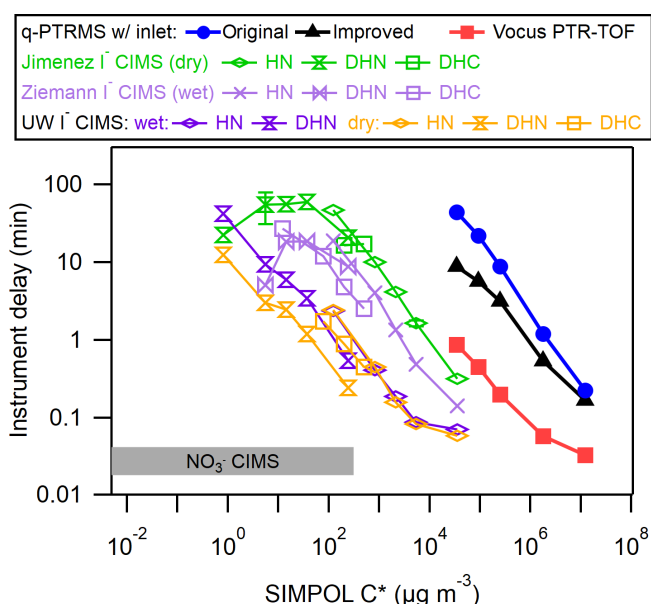
Figure 4. Delay times for a variety of organic molecules as a function of saturation vapor concentration ( C^* , \mu\text{g m}^{-3} ), compared with previous IMR designs including a q-PTRMS, Vocus PTR-ToF-MS, and several I^- CIMS instruments with different IMRs. The delay time in a nitrate ( \text{NO}_3^- ) CIMS is also shown for comparison. The organic molecules are described in Table S1 in the Supplement.
