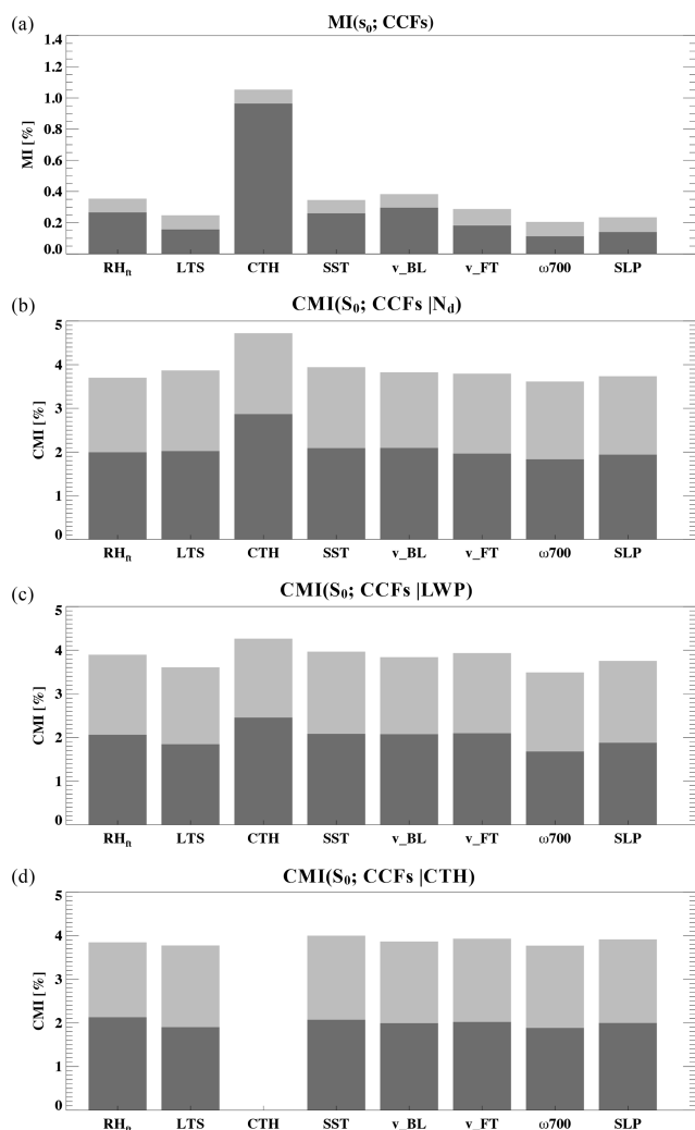
Figure 1. (a) Mutual information (MI; dark gray) for S_0 and eight meteorological factors (MFs; denoted as cloud controlling factors, CCFs), including RH_h , LTS, CTH, SST, BL, and FT winds, 700 hPa vertical velocity ( \omega_{700} ), and sea level pressure (SLP). (b–d) Conditional MI (CMI; dark gray) for S_0 and the 8 MFs, conditioned by N_d , LWP, and CTH, respectively. Noise-CMI (light gray) is represented by the (conditional) mutual information between MFs and randomly permuted S_0 sample space (effectively noise).
