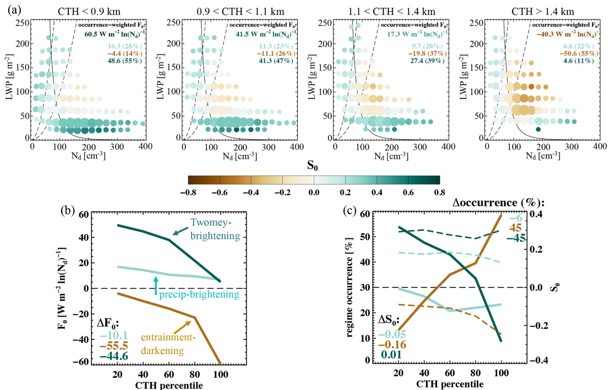
Figure 6. (a) As in Fig. 2 but conditioned on cloud-top height (CTH) quartiles. Occurrence-weighted mean (b) F_0 and (c) regime-mean S_0 (dashed curves) and regime-occurrence (solid curves) of the three albedo susceptibility regimes (defined in Fig. 2) as a function of CTH; increment of 20th percentile.
