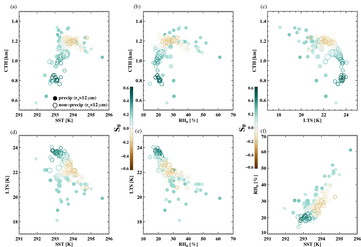
Figure 4. Mean meteorological/cloud state conditions associated with each LWP– N_d bin in Fig. 2, in the space of (a) CTH–SST, (b) CTH– RH_{ft} , (c) CTH–LTS, (d) LTS–SST, (e) LTS– RH_{ft} , and (f) RH_{ft} –SST. Size and color of the circles represent the frequency of occurrence and the mean S_0 of that LWP– N_d bin, respectively, as shown in Fig. 2. Precipitating clouds (based on a r_c threshold of 12 \mu\text{m} ) and non-precipitating clouds are indicated by filled and open circles, respectively.
