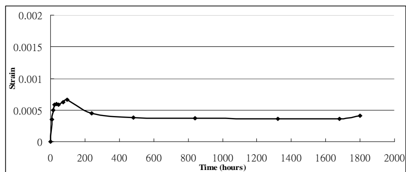
Figure 3.8 Drying shrinkage (Group 12-3)
