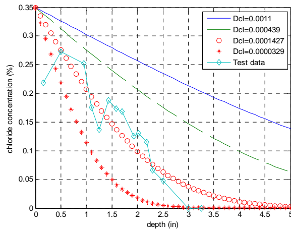
Figure 5.14 Chloride concentration profiles (Bridge G22-BJ; shoulder lane)
