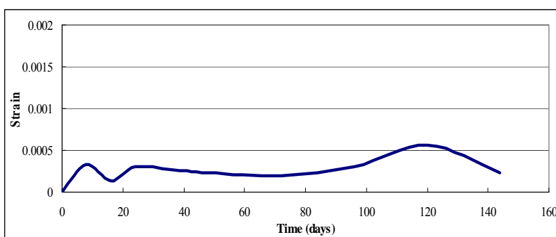
Figure 3.6 Drying shrinkage (Group 9-3)
