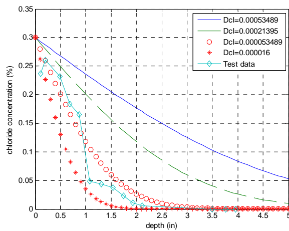
Figure 5.15 Chloride concentration profiles (Bridge G22-BJ; traffic lane)
