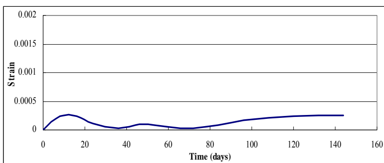
Figure 3.5 Drying shrinkage (Group 9-1)
