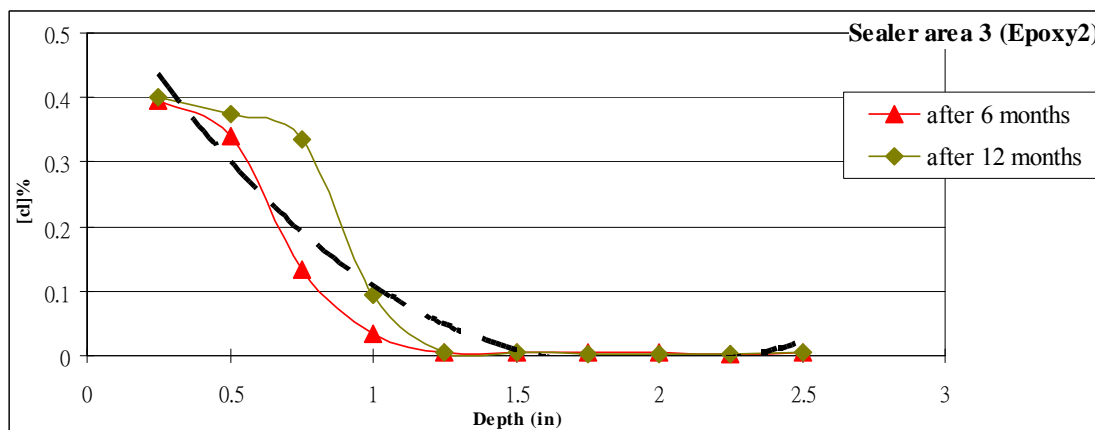
Figure 7.9 Chloride concentration (Epoxy 2)
