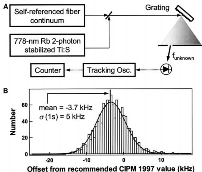
Fig. 6. Frequency metrology with the self-referenced frequency comb. (A) Experimental setup to measure the ^5S_{1/2} (F = 3) \rightarrow ^5D_{5/2} (F = 5) two-photon transition in ^{85}\text{Rb} with a self-stabilized frequency comb. (B) Histogram of one set of measurements in relation to the recommended CIPM (1997) value of 385,285,142,378 \pm 5.0 kHz for the rubidium transition. The standard deviation at the 1-s gate time is 5 kHz, which is an absolute uncertainty of 1 part in 10^{11} .
