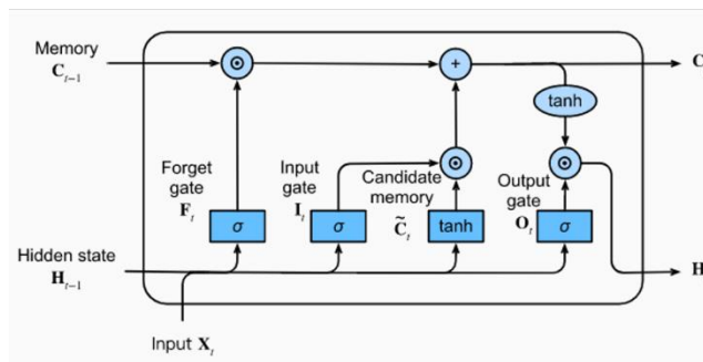
Fig. 3 LSTM Architecture [14]
