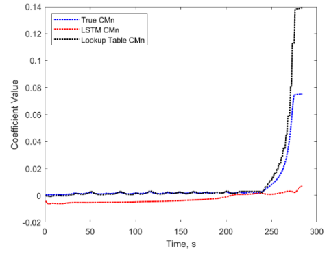
b.) Yawing Moment Coefficient
