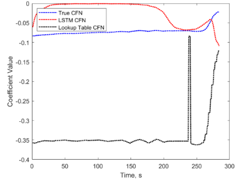
b.) Normal Force Coefficient
