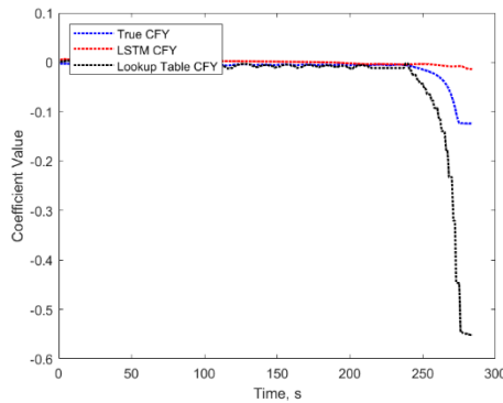
c.) Lateral Force Coefficient
