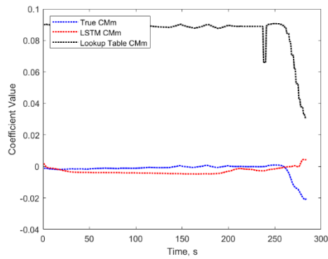
b.) Pitching Moment Coefficient
