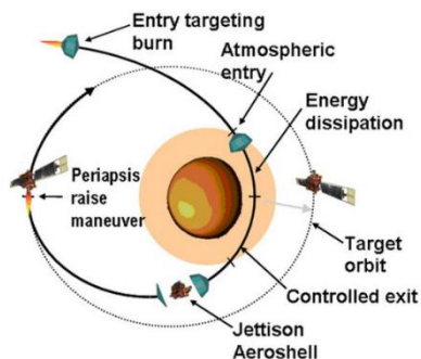
Fig. 1 Notional Aerocapture Maneuver [4]
