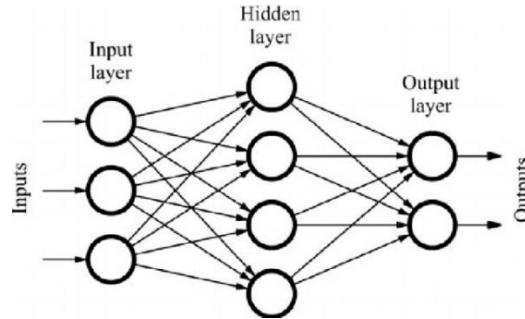
Fig. 2 FFNN Architecture [10]
