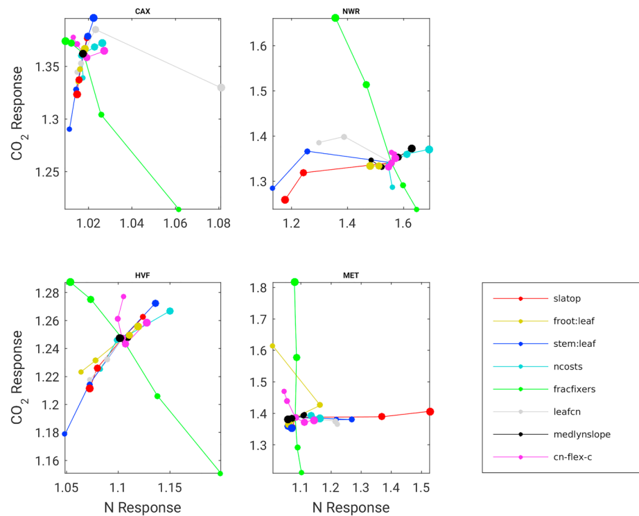
Figure 4. Influence of parametric variation on the model response (fertilized/control) to 15 years of 500ppm \text{CO}_2 and +5\text{Kg m}^{-2} \text{y}^{-1} N fertilization on gross primary productivity (GPP). Note changes in scale between plots to show detail.
