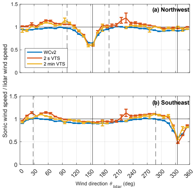
Figure 13. Ratio of mean wind speed from the northwest (a) and southeast (b) sonic anemometers versus the 2 min WINDCUBE ® V2 (WCv2) profiling lidar (blue) and 2 s (red) and 2 min (yellow) virtual tower stares (VTS) at the BAO tower, for all heights (50 m intervals from 50 to 150 m), in 10° bins as determined by the respective lidar's wind direction. WCv2 comparisons cover the entire period from 12 March to 31 May 2015, and VTS comparisons at the BAO tower span the 3-day period from 21 to 24 March 2015. Vertical dashed lines denote the largest tower-wake boundaries in Table 1 (100–189 and 288–28°).
