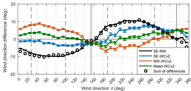
Figure 15. Difference in 2 min mean wind direction between the sonic anemometers on the two booms (southeast minus northwest: solid black; mean of southeast and northwest: green) in 10^\circ bins as determined by the southeast sonic anemometers' wind directions and the WINDCUBE ® V2 profiling lidar at 50, 100, and 150 m (southeast sonic anemometers minus WCv2: blue; northwest sonic anemometers minus WCv2: red), in 10^\circ bins as determined by the WCv2 wind directions. Black circles are the sum of the differences between the sonic anemometers and the WCv2. Vertical solid black line denotes the orientations of the booms, and vertical dashed lines denote the largest tower-wake boundaries in Table 1 (100–189 and 288–28°).
