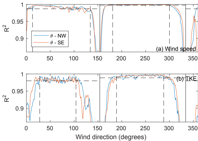
Figure 9. Coefficient of determination, R^2 , of the 2 min mean wind speeds (a) and 20 min TKE (b) measured by the southeast and northwest sonic anemometers at all heights for the full 3 months of measurements, binned into 1^\circ wind direction intervals, and smoothed with a running mean of 3^\circ . The boom orientations are shown in solid black vertical lines, and dashed vertical lines denote the wakes as determined by the limits in the horizontal dashed lines. The blue line uses the wind directions from the northwest sonic to identify the wake formed around the southeast sonic anemometer near 334^\circ , and the red line uses the wind directions from the southeast sonic anemometer to identify the wake around the northwest sonic anemometer near 154^\circ .
