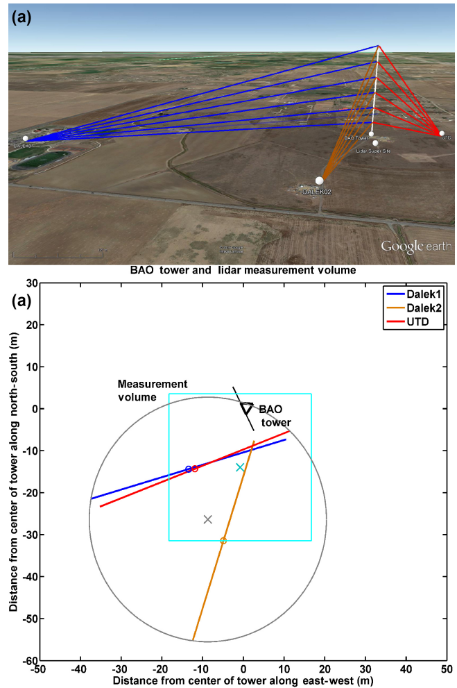
Figure 3. Top: schematic of the triple-Doppler virtual tower stares (VTS) of the three Leosphere 200S scanning lidars (Dalek1: blue, Dalek2: brown, and UTD: red), as they stare at the BAO tower's six levels of sonic anemometers at 50, 100, 150, 200, 250, and 300 m a.g.l. The WCv2 is also shown near the BAO tower. Bottom: bird's-eye view of the measurement volume (cyan box, with x at the center) resulting from the range gates of the three scanning lidars, drawn with circles at the centers of the beams, to scale. The footprint of the beams of the VTS is shown in the black circle, with an x at the center.
