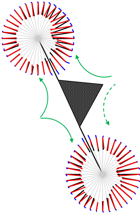
Figure 17. The vector representations of the average winds measured by the sonic anemometers at all heights (red) and the 2 s VTS (black), on the tower layout, with the vector of the perturbation in blue. Green curved arrows summarize the general trends around the sides of the tower with consistent behavior, with a dashed line indicating less consistent behavior in that quadrant.
