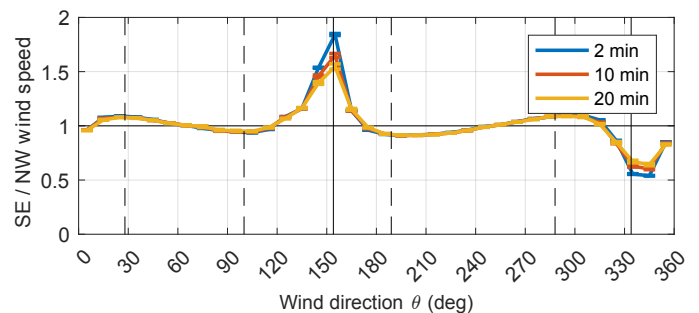
Figure 11. Ratio of southeast to northwest sonic anemometers' wind speed, calculated over 2 min (blue), 10 min (red), and 20 min (yellow) intervals, using data from all heights of the BAO tower. Vertical solid lines denote the boom orientation angles, and the vertical dashed lines denote the largest tower-wake boundaries in Table 1 ( 100 – 189 and 288 – 28^\circ ).
