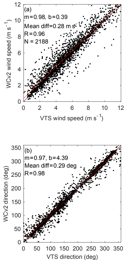
Figure 12. (a) Scatterplot of 25 s wind speeds from the WINDCUBE ® V2 (WCv2) and accumulations of wind speed from the virtual tower stars (VTS) over the lidar super site, using data from 9 days of the three 200S lidars performing coordinated stars over the supersite location at heights of 100 to 200 m above ground with 20 m increments (number of points, N = 2188 ). The black dashed line is the one-to-one line, and the red line is the line of best fit, with slope, m , and intercept, b , as noted. The mean difference between measurements, and correlation coefficient, R , are also shown. (b) Same as in panel (a), but for wind direction.
