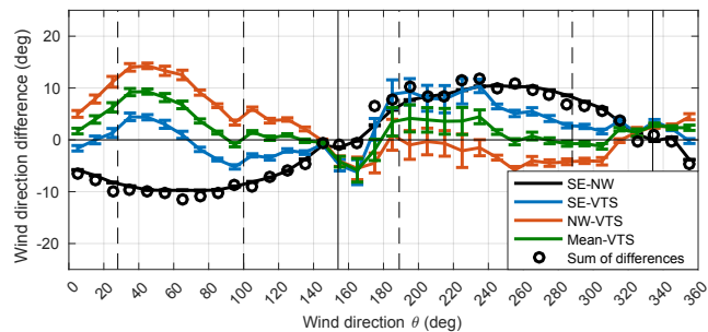
Figure 16. Same as Fig. 15, but showing the difference in wind direction between the 2 s sonic anemometer and virtual tower stare (VTS) measurements.
