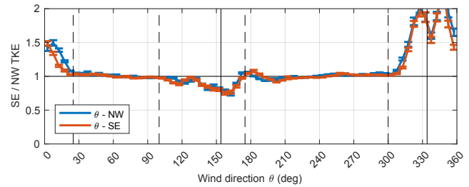
Figure 7. Ratio of 20 min turbulent kinetic energy (TKE) from the southeast versus northwest sonic anemometers at all six heights for the full 3 months of measurements during XPIA, in 5° wind direction bins as determined by the northwest (blue) and southeast (red) sonic anemometers. Solid vertical lines indicate the orientations of the booms at 154 and 334° from north and dashed vertical lines indicate the boundaries of the wake, defined by the TKE increase, at 100–175 and 300–25°. Error bars represent 1 standard deviation of the mean.
