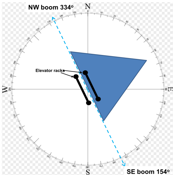
Figure 1. Plan view schematic of the BAO tower as the blue equilateral triangle, with the northwest and southeast booms depicted and their orientations relative to north. The interior elevator track and exterior carriage track are also shown on the southwest face.
