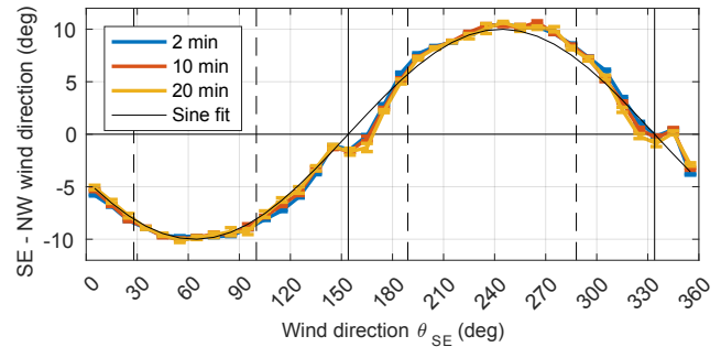
Figure 14. Difference in wind direction between the sonic anemometers on the two booms (southeast minus northwest), calculated over 2 min (blue), 10 min (red) and 20 min (yellow) intervals, using data from all six heights of the BAO tower, in 10° bins as determined by the southeast sonic anemometers' wind directions. The thin black line is the approximate sine-function fit, \Delta\theta = 10\sin(\theta - 154) . Vertical solid lines denote the boom orientation angles, and the vertical dashed lines denote the largest tower-wake boundaries in Table 1 (100–189 and 288–28°).
