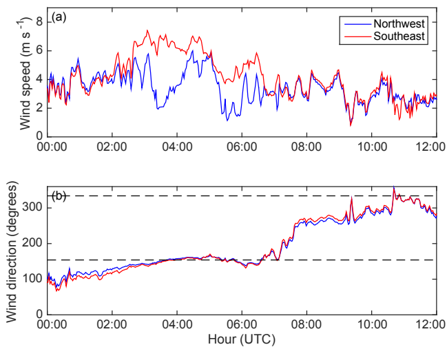
Figure 4. Two-minute average wind speed (a) and direction (b) from the 50 m sonic anemometers on the northwest boom (blue) and southeast boom (red), from 00:00 to 12:00 UTC on 4 April 2015. Dashed lines in (b) show the angles of the boom orientations at 154 and 334° from north.
