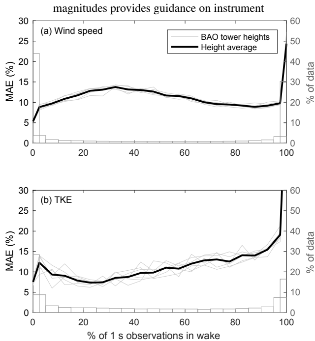
Figure 18. The mean absolute error (in percent) for the 2 min mean wind speed (a) and 20 min TKE (b) versus percentage of 1 s averages of the 20 Hz sonic anemometer observations which are in the tower wake and have been removed from the 2 or 20 min intervals. All six BAO tower measurement heights are shown in gray, with the mean over all heights in black. The distribution of all observations that contribute to each bin (averaged over all heights) is shown in bars, with labels on the right axis of both plots for the respective time intervals.
