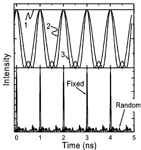
FIG. 4. Schematic of the pulse train generated by locking the phase of simultaneously oscillating modes. The upper panel shows the output intensity as the number of modes is increased from 1 to 2 to 3. The lower panel shows the result for 30 modes, both phase locked and with random phases. The mode spacing is 1 GHz.
