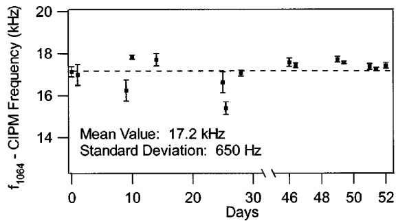
FIG. 19. Summary of direct rf to optical measurement of f_{1064} plotted with respect to the CIPM recommended value. The +17.2 kHz average of all measurements is shown by the dashed line.
