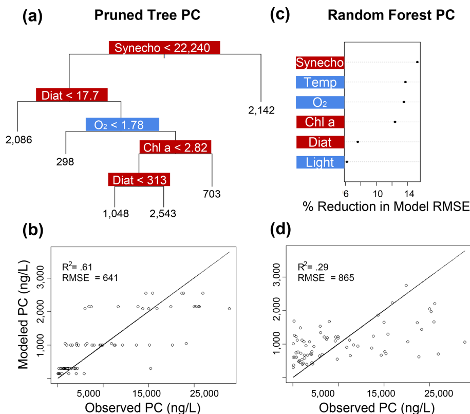
Figure 7. Classification and regression tree (CART) and random forest analyses of selected IPL classes (PC). Panel (a) indicates a summary of primary predictors in the best-fit CART (i.e., pruned tree), whereas panel (b) shows model performance via adjusted R^2 and RMSE. Panel (c) displays random forest variable importance in the prediction of IPL classes as defined by percent reduction in RMSE, whereas panel (d) shows model performance via adjusted R^2 and RMSE. Environmental variables are depicted in blue, whereas biological variables are shown in red for both analyses.
