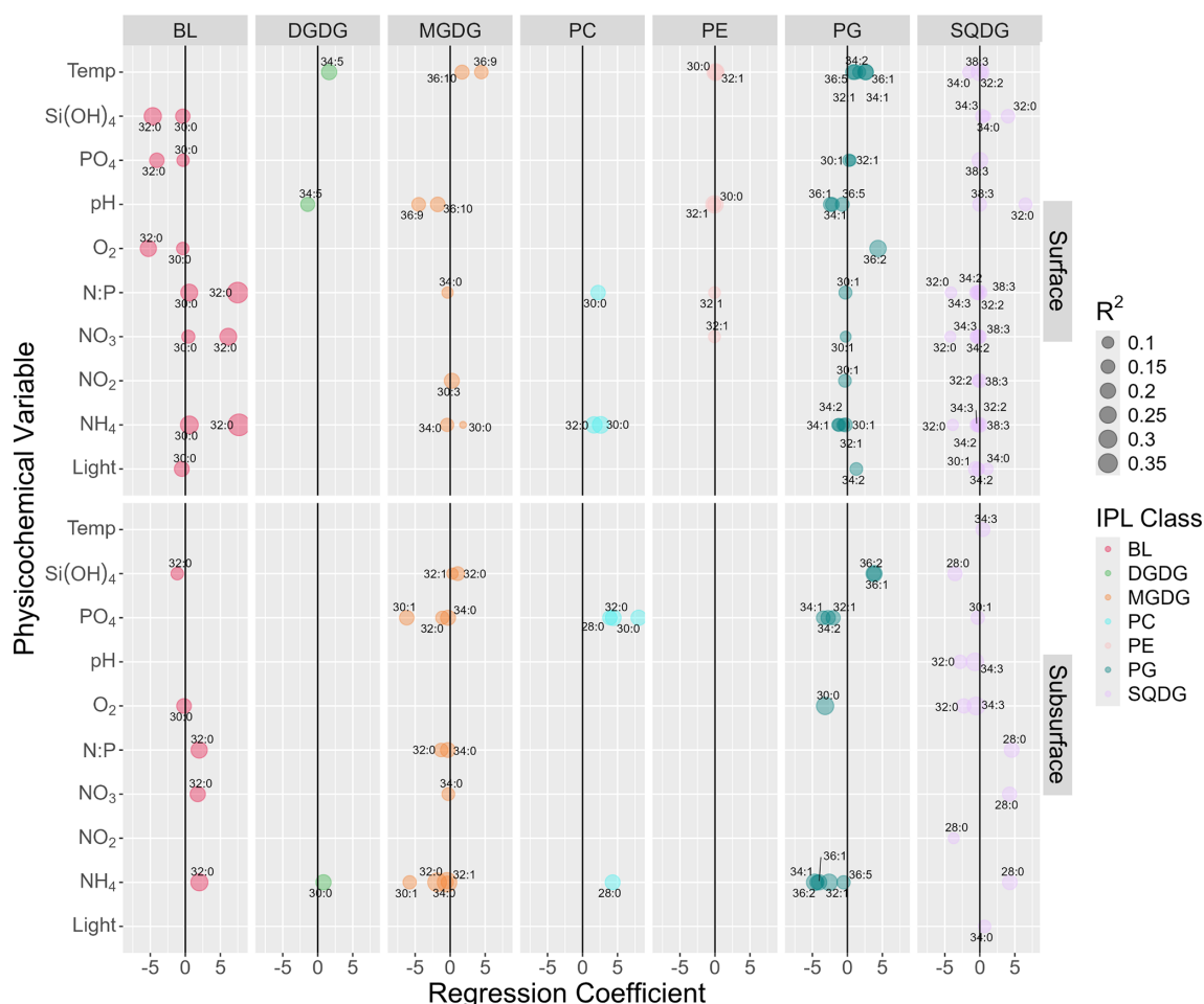
Figure 3. Summary of multiple linear regression analysis between the abundances of major IPL molecules ( > 2.5\% of total IPL pool) and physicochemical parameters showing only statistically significant ( p < 0.05 ) linear responses after controlling for the false discovery rate using a 0.1 alpha cutoff on adjusted p values. The size of circles indicates the magnitude of the linear-regression-adjusted R^2 . The upper and lower panels represent surface and subsurface waters, respectively. Numbers next to circles indicate the total number of carbon atoms and double bonds in core fatty acid chains.
