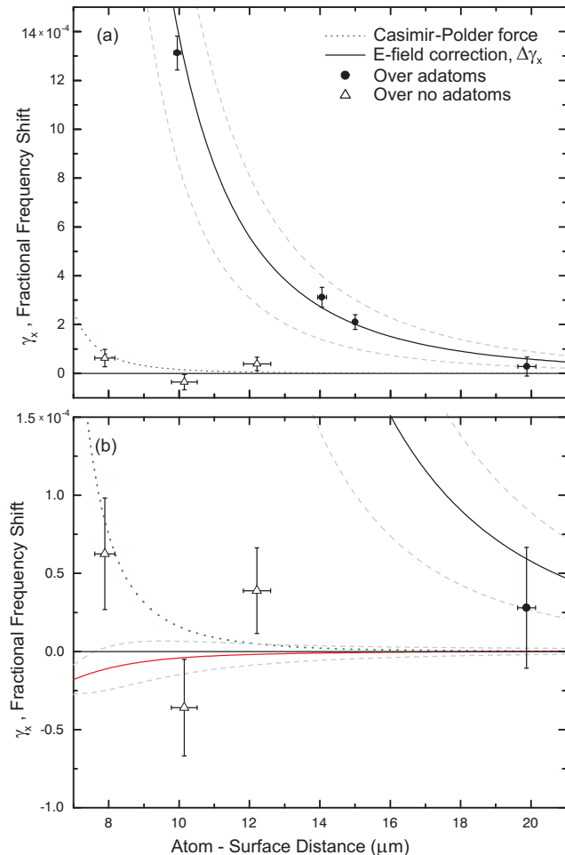
FIG. 5: (Color online). (a) The measured fractional frequency shift for two separate surface locations. The filled circles are data taken directly over 7 \times 10^7 adsorbed atoms, and the solid black line is the shift predicted from electric-field measurements. The dashed gray lines represent error bounds obtained from field-gradient measurements. The open triangles are data taken over a ‘clean’ surface location (no adatoms) where the electric-field correction is consistent with zero (solid red line in (b)). The correction to data taken over a clean spot is frequently small enough to exhibit a two-component power law dependence for which the correction may, in fact, be slightly negative. The expected Casimir-Polder shift is shown with a green dotted line.
