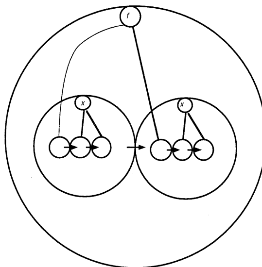
Figure 1. VEX representation of the Y combinator
