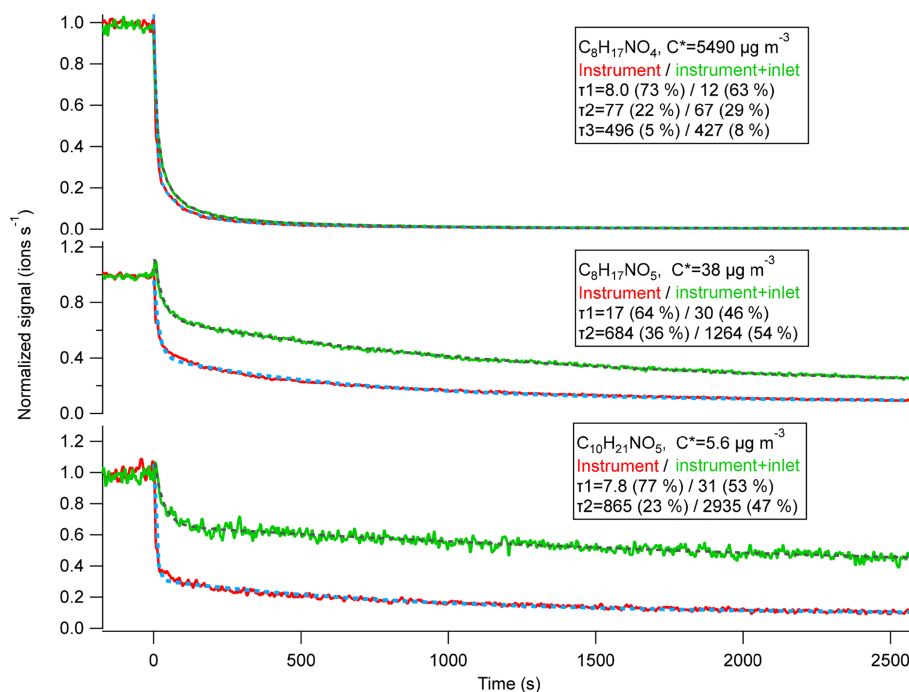
Figure 1. Example instrument-only (red, solid lines) and instrument + FEP tubing (green, solid lines) depassivation responses for three different hydroxynitrates observed by the Jimenez I-CIMS. In all cases multi-exponential decays were observed (dashed line fits), with a substantial initial fast decay, followed by a much slower decrease in the signal. Note these decays have different timescale ( \tau ) values. The percentages in parentheses are fractions of original signals associated with each \tau .
