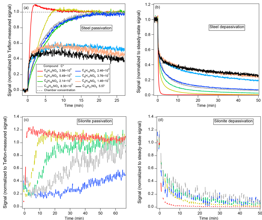
Figure 4. Examples of passivation and depassivation of stainless steel ( a , b ) for C_6 – C_{10} HN and DHN and Silonite ( c , d ) for C^* > 10^2 \mu\text{g m}^{-3} HN and DHN, where curves were binomially smoothed across 10 points for visual clarity. The stainless-steel data were measured by the CU (Ziemann) CIMS. The Silonite data were measured with the UW CIMS, and the gaps were due to periodic background sampling. Note that the starting signals for ( c ) are not zero, due to compounds that remained in the instrument.
