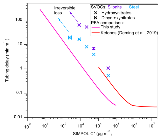
Figure 5. Stainless-steel and Silonite depassivation delay times measured for a series of HNs and DHNs after equilibration with a chamber filled with alkanols and S/IVOCs, and compared with PFA modeled delays for 4 \text{ L min}^{-1} flows. Only compounds with 100 % transmission efficiency through stainless steel and Silonite compared to Teflon tubing are shown. DHCs were not included in delay calculation due to relatively low S/N ratios in these experiments. The transmission became lower than 100 % for DHCs with C^* < 10^2 \mu\text{g m}^{-3} through steel and C^* < 10^3 \mu\text{g m}^{-3} through Silonite. Example error bars (smaller than marker) were propagated from exponential fits.
