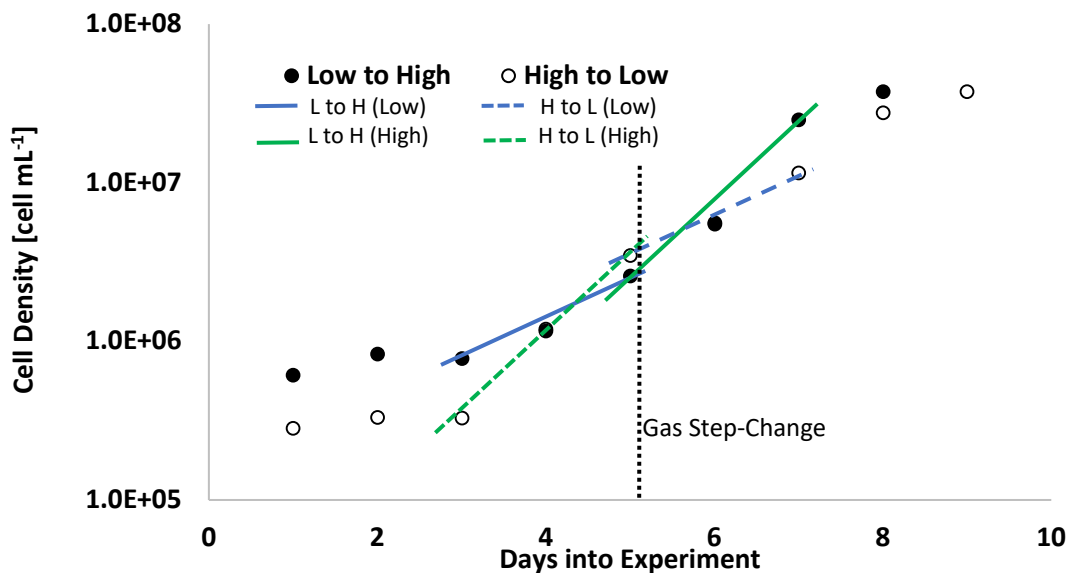
Figure 53. Cell counts plotted on a semi-log plot to identify the onset exponential growth. Those areas associated with exponential growth are highlighted for each gas step-change case (line type), with each gas level indicated by color.
