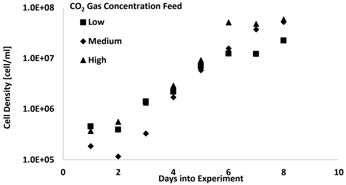
Figure 98. Daily cell counts for each steady-state CO 2 concentration plotted on a semi-log plot over experiment duration
