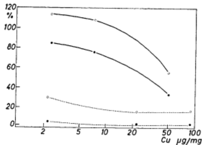
Figure 14. Respiration and photosynthesis of cells treated with copper under aerobic and anaerobic conditions. Ordinate: Rates of respiration and photosynthesis as percentage of control. Abscissa: Amount of copper applied in \mu\text{g}/\text{mg} DW cells. Open circles = Respiration, Closed circles = Photosynthesis; Full lines = Aerobic conditions; Dotted lines = Anaerobic conditions (selected from (McBrien and Hassall 1967)).
