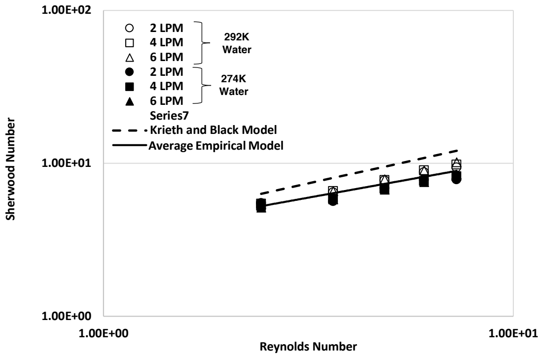
Figure 63. Correlation of non-dimensional numbers for oxygen transport at laminar flow conditions. Developed oxygen transport model and the Kreith & Black model are shown for comparison.
