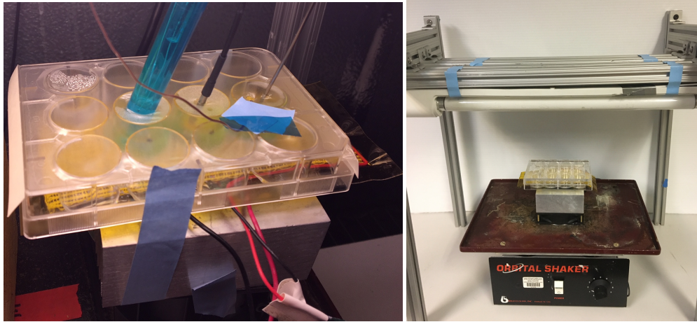
Figure 24. pH, dissolved oxygen, and temperature probes inserted through membrane (left image). Well-plate and stand on top of orbital shaker table under fluorescent light bank (right image).
