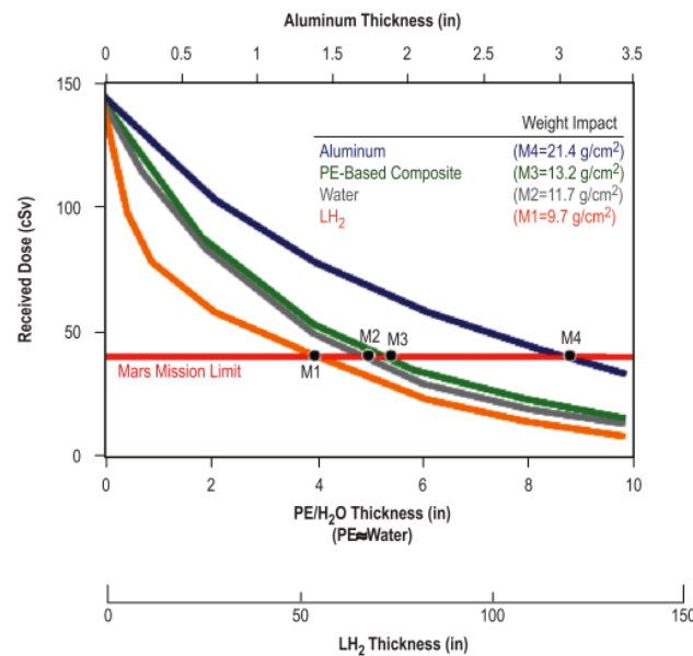
Figure 86. Received dose versus the thickness of PEM, H 2 O, and H 2 for radiation shielding. The mass impact is also indicated (selected from (Barghouty and Thibeault, 2006)).
