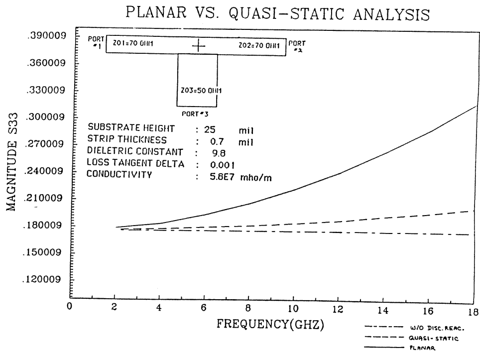
Figure 5.5: Planar analysis vs. quasi-static analysis for the reflection at the branch line of the tee-junction.
