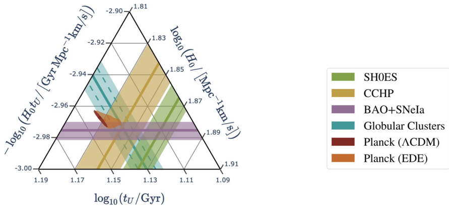
Fig. 45 Triad plot “new cosmic triangle”: 68% confidence level marginalized constraints on the new cosmic triangle: the triad corresponding to the age of the Universe and the Hubble constant (upper left) is shown. Note that all points in the figure sum up to 0, while the ticks in the axes determine the direction of equal values for each axis. Note that absolute ages of GCs are consistent with the model-dependent Planck18 value. Image reproduced with permission from Bernal et al. (2021), copyright by APS
