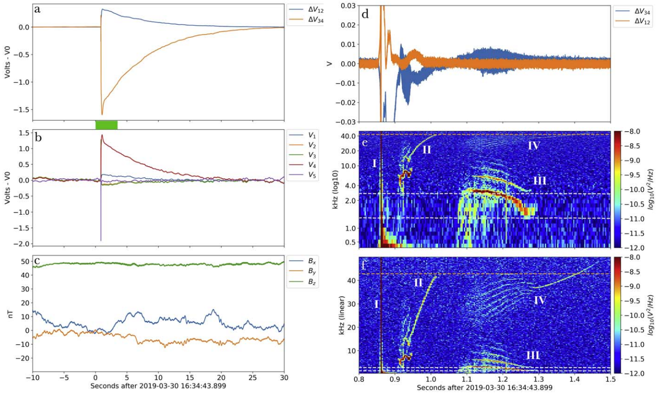
Figure 5. Debris-producing impact event signatures. (a), (b), (c) follow the same format as Figure 1 (a), (b), (c). (d) Differential voltage data from V_{12} and V_{34} , over \sim 0.7 s. (e) Windowed power spectra of data in (a), with logarithmic frequency axis. (f) Windowed power spectra of data in (d), with linear frequency axis. White dashed lines indicate the local electron cyclotron frequency (lower) and twice the local electron cyclotron frequency (upper). The orange dashed line indicates the local electron plasma frequency as it would appear when aliased into the observed signal.
