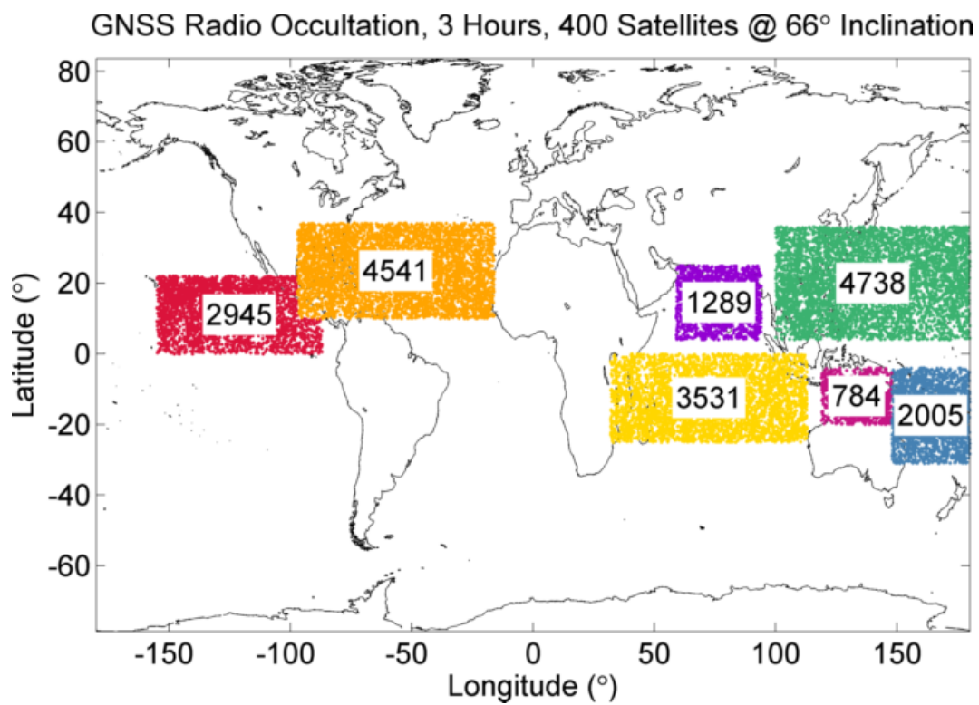
Figure 4.17: Three-hour coverage of cyclone regions using the simulated 400 RO satellite constellation.
