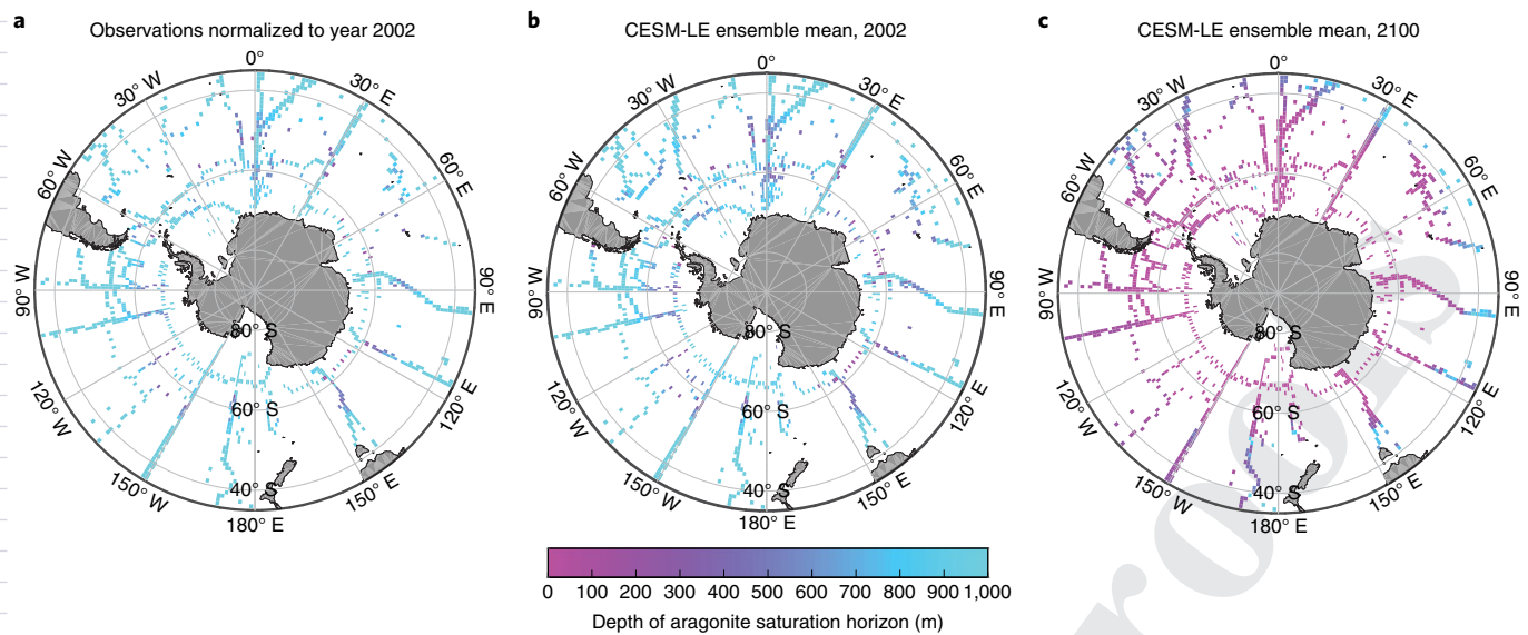
Fig. 1 | Depth of aragonite saturation horizon. a–c , Shows depth of the aragonite saturation horizon from GLODAPv2 bin-averaged DIC (normalized to year 2002) and alkalinity, as well as hydrography data from World Ocean Atlas (WOA 2009) sub-sampled at the GLODAPv2 data locations ( a ), CESM-LE in 2002, corrected for model bias using hydrographic observations (see Methods) ( b ), and CESM-LE in 2100 ( c ). Model projections are displayed in 1^\circ \times 1^\circ grid cells where there are sufficient GLODAPv2 data to identify a present-day saturation horizon.
