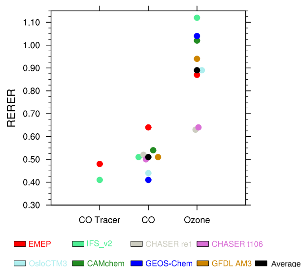
Figure 2. Model-calculated annual CO tracer, CO and ozone RERER (Response to Extra-Regional Emission Reductions) values for Europe calculated by the models; see equation in Sect. 4. Similar RERER values have been displaced horizontally.
