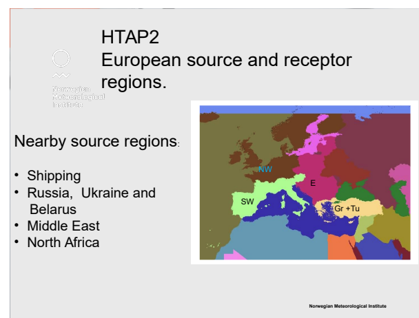
Figure 1. HTAP2 regions. The European land areas are further subdivided: NW is western Europe, north of the Alps; SW is western Europe south of the Alps; E is eastern Europe and Gr + Tu is Greece and Turkey.
