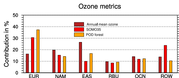
Figure 6. Contributions to ozone metrics annual mean ozone, SOMO35 and \text{POD}_1 forest in percent (where BASE–GLOALL represents 100 %) as calculated by the EMEP_rv48 model. The metrics have been scaled so that the difference between the BASE–GLOALL (20 % anthropogenic emission reductions) calculations is 100 % (the sum of EUR, NAM, EAS, RBU, OCN and ROW is 100 %).
