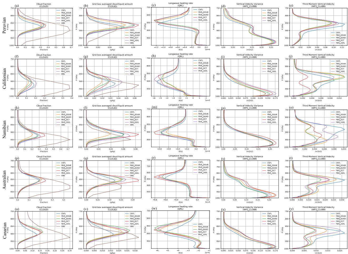
Figure 8. Spatial- and temporal-averaged profiles of (a) cloud fraction, (b) cloud liquid water amount, (c) longwave heating rate, (d) second moment vertical velocity ( \overline{w^2} ), and (e) third moment vertical velocity ( \overline{w^3} ) in the Peruvian region (defined in Table 3) from the simulations of Energy Exascale Earth System Model (E3SM)-Framework for Improvement by Vertical Enhancement (FIVE). (f–j) are the same as (a–e) but in the Californian region. (k–o) are the same as (a–e) but in the Namibian region. (p–t) are the same as (a–e) but in the Australian region. (u–y) are the same as (a–e) but in the Canarian region. CNTL, control run; DOUB, double; OCT, octuple; QUAD, quadruple; 16XL, sexdecuple.
