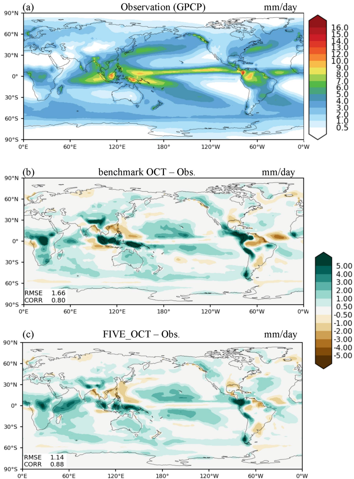
Figure 11. (a) Precipitation from Global Precipitation Climatology Project (GPCP) data set averaged from 1979 to 2014. (b) The differences of precipitation between Energy Exascale Earth System Model (E3SM) benchmark octuple (OCT) and the observation. (c) The differences of precipitation between FIVE_OCT and the observation. The bottom two rows of (b and c) display the evolution of the geographical biases, root mean squared errors (RMSE), and correlation coefficients (CORR) of the OCT and FIVE_OCT simulations computed relative to the observation.
