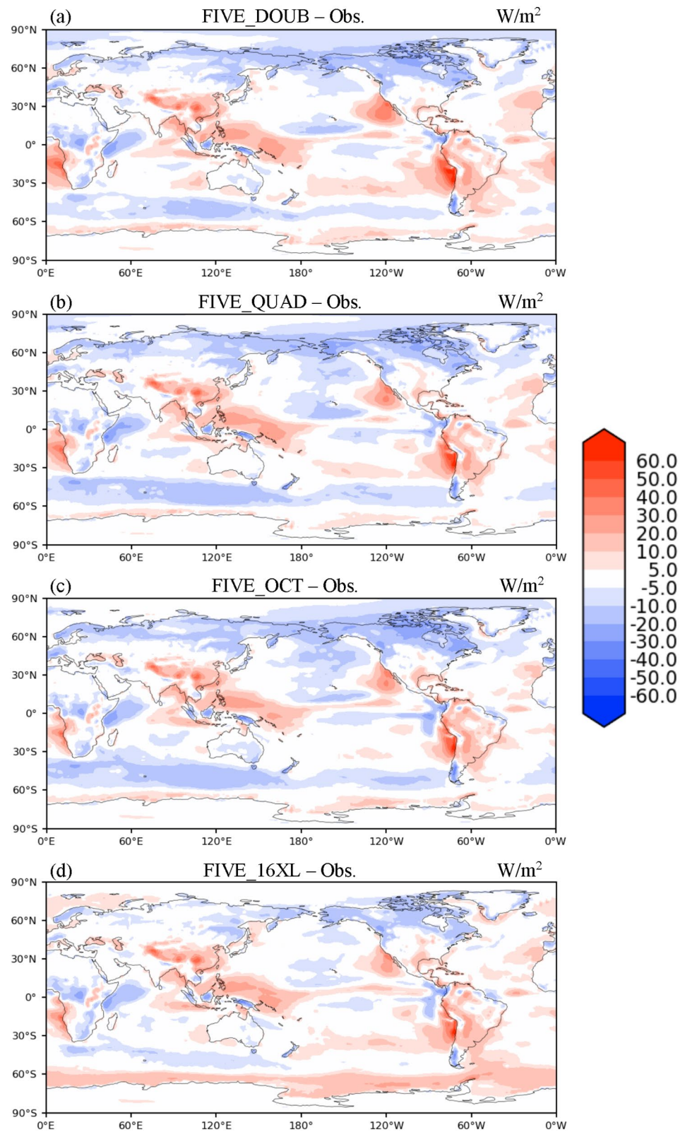
Figure 7. (a) The differences of shortwave cloud radiative effect between FIVE_DOUB and the observation (Figure 3a). (b–d) are the same as (a) but for FIVE_QUAD, FIVE_OCT, and FIVE_16XL, respectively. DOUB, double; FIVE, Framework for Improvement by Vertical Enhancement; OCT, octuple; QUAD, quadruple; 16XL, sexdecuple.
