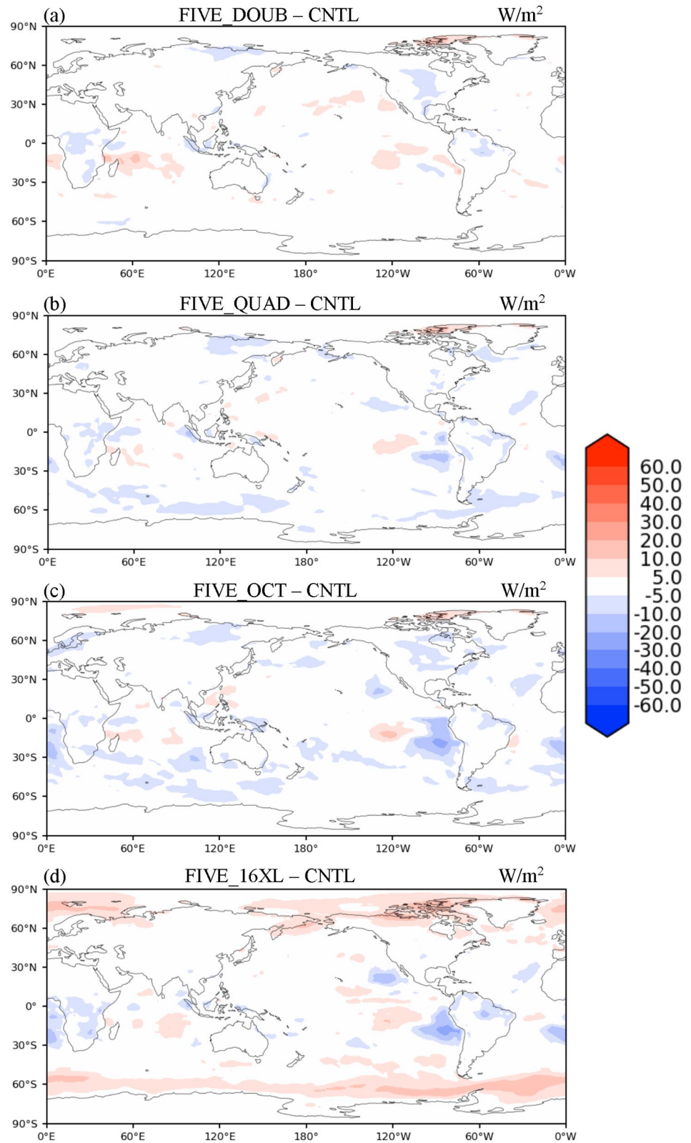
Figure 5. (a) The differences of shortwave cloud radiative effect between FIVE_DOUB and CNTL (Figure 3b). (b–d) are the same as (a) but for FIVE_QUAD, FIVE_OCT, and FIVE_16XL, respectively. CNTL, control run; DOUB, double; FIVE, Framework for Improvement by Vertical Enhancement; OCT, octuple; QUAD, quadruple; 16XL, sexdecuple.
