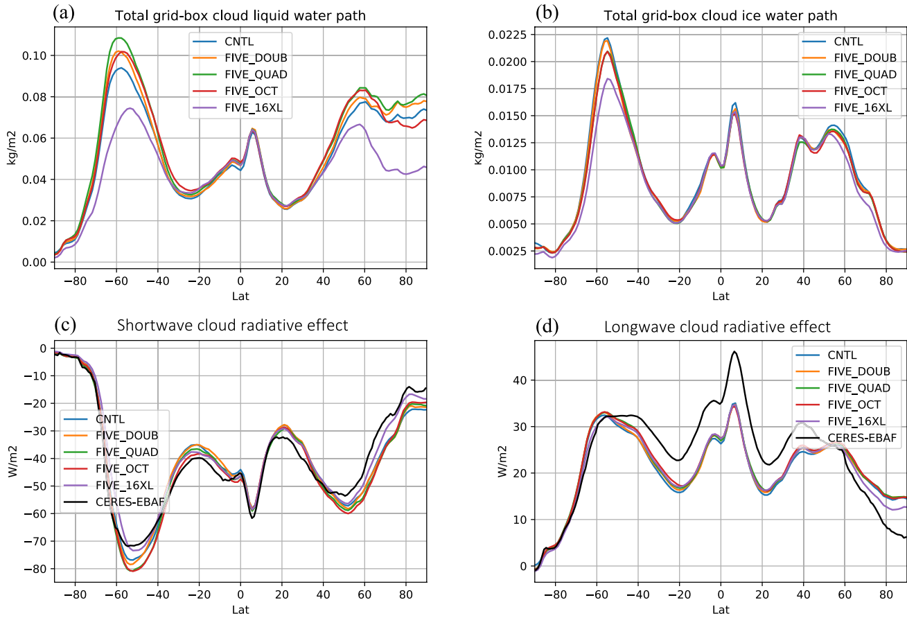
Figure 6. The zonal average of (a) cloud liquid water path ( \text{kg}/\text{m}^2 ), (b) cloud ice water path ( \text{kg}/\text{m}^2 ), (c) shortwave cloud radiative effect ( \text{W}/\text{m}^2 ), and (d) longwave cloud radiative effect ( \text{W}/\text{m}^2 ) from the simulations of Energy Exascale Earth System Model (E3SM)-Framework for Improvement by Vertical Enhancement (FIVE). CERES-EBAF is the Clouds and the Earth's Radiant Energy System (CERES) Energy Balanced and Filled (EBAF) top-of-atmosphere (TOA) data product averaged from 2000 to 2015. CNTL, control run; DOUB, double; OCT, octuple; QUAD, quadruple; 16XL, sexdecuple.
