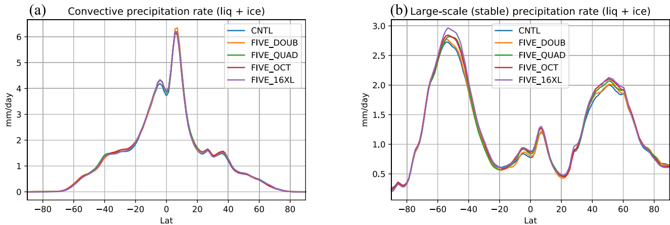
Figure 12. The zonal average of (a) convective precipitation rate (mm/day) and (b) large-scale precipitation rate (mm/day) from the simulations of Energy Exascale Earth System Model (E3SM)-Framework for Improvement by Vertical Enhancement (FIVE). CNTL, control run; DOUB, double; OCT, octuple; QUAD, quadruple; 16XL, sexdecuple.
