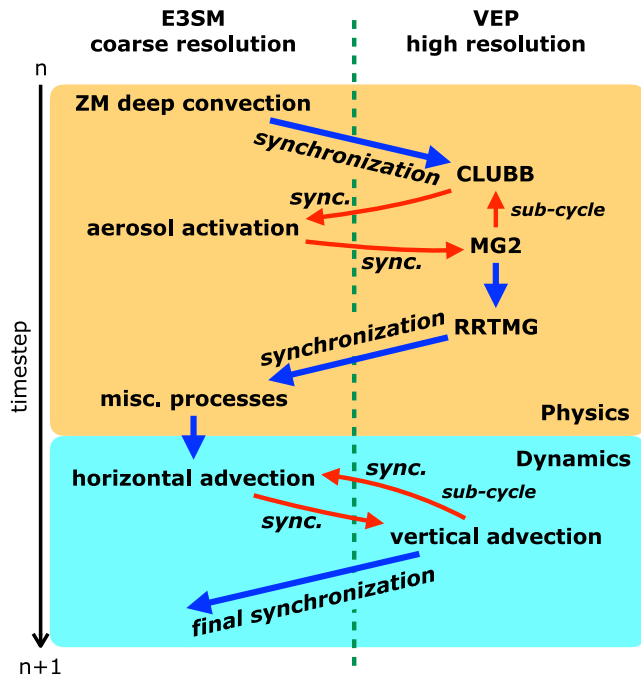
Figure 1. Schematic of the sequence of the processes between the host model (i.e., Energy Exascale Earth System Model [E3SM]) and selected schemes for vertically enhanced physics (VEP). The sequence of processes in the host model is Zhang-McFarlane deep convection scheme (host model)→synchronization→Cloud Layers Unified By-Binormals (CLUBB) turbulence parameterization (VEP)→Morrison and Gettelman microphysics scheme version 2 (MG2) microphysics scheme (VEP)→(CLUBB and MG2 sub-cycle)→Rapid Radiative Transfer Model for GCMs (RRTMG) radiation schemes (VEP)→synchronization→Miscellaneous other atmospheric processes (host model)→horizontal advection (host model)→synchronization→vertical advection (VEP)→(horizontal advection and vertical sub-cycle)→final synchronization.
