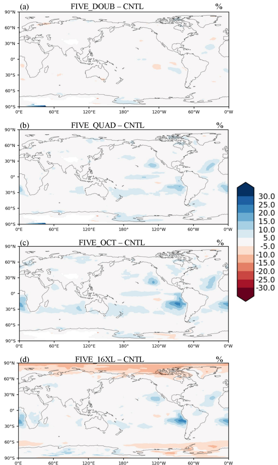
Figure 4. (a) The differences of low-level cloud amount between FIVE_DOUB and CNTL (Figure 2b). (b–d) are the same as (a) but for FIVE_QUAD, FIVE_OCT, and FIVE_16XL, respectively. CNTL, control run; DOUB, double; FIVE, Framework for Improvement by Vertical Enhancement; OCT, octuple; QUAD, quadruple; 16XL, sexdecuple.
