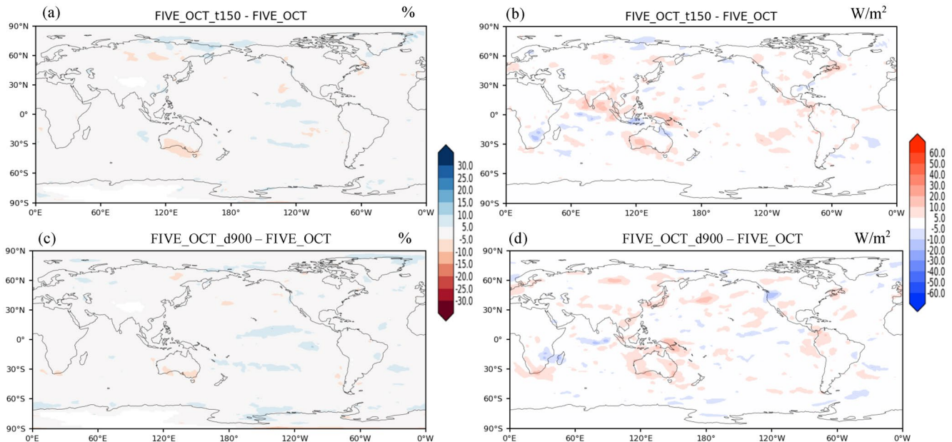
Figure 14. (a) The differences of low-level cloud amount between FIVE_OCT_t150 and FIVE_OCT. (b) The differences of shortwave cloud radiative effect between FIVE_OCT_t150 and FIVE_OCT. (c and d) are the same as (a and b), respectively, but the differences between FIVE_OCT_d900 and FIVE_OCT. The results are 2 years average. FIVE, Framework for Improvement by Vertical Enhancement; OCT, octuple.
