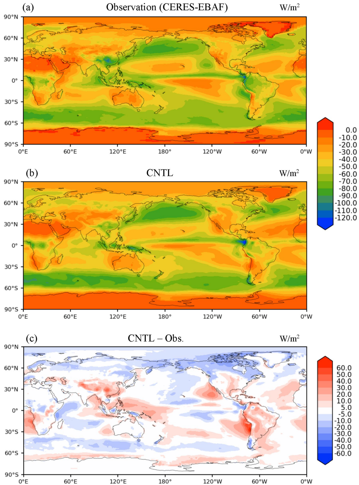
Figure 3. (a) Shortwave cloud radiative effect (SWCRE) from the Clouds and the Earth’s Radiant Energy System (CERES) Energy Balanced and Filled (EBAF) top-of-atmosphere (TOA) data product averaged from 2000 to 2015. (b) Averaged SWCRE in the control run (CNTL). (c) The differences of SWCRE between CNTL and the observation.
