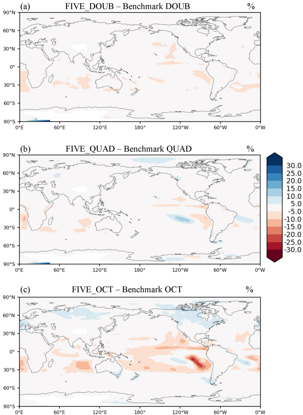
Figure 9. (a) The differences of low-level cloud amount between Energy Exascale Earth System Model (E3SM) benchmark DOUB and FIVE_DOUB (Figure 1b). (b) is the same as (a) but between QUAD and FIVE_QUAD. (c) is the same as (a) but between OCT and FIVE_OCT. DOUB, double; FIVE, Framework for Improvement by Vertical Enhancement; OCT, octuple; QUAD, quadruple; 16XL, sexdecuple.
