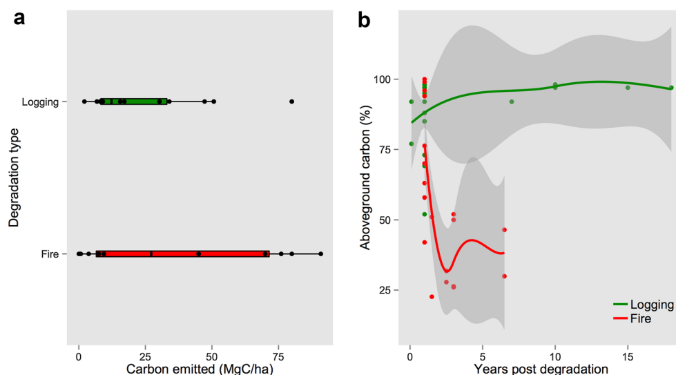
Fig. 2 a Short-term (1 year or less) carbon emissions after logging (average = 23.5 MgC/ha, minimum = 2.1 MgC/ha, maximum = 80.0 MgC/ha), and fire disturbance (average = 36.3 MgC/ha, minimum = 0.03 MgC/ha, maximum = 90.9 MgC/ha). b Aboveground carbon stock (in % of original/undisturbed forest) trajectories after logging (green) and fire (red), collected from 31 studies reporting carbon or biomass in degraded forests. Shaded areas represent 95% confidence intervals of loess smoothing
