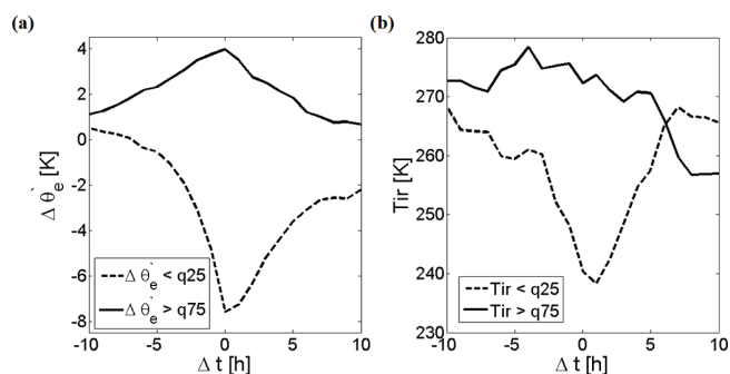
Figure 13. Ensemble analysis for (a) \Delta\theta'_e and (b) T_{\text{ir}} considering 10 h before and 10 h after the event's onset. The cases where \Delta\theta'_e at the event's onset is less than the 25th percentile (dashed lines) and more than the 75th percentile (full lines) are shown. In total, 72 cases were considered in the analysis (36 cases for each condition).
