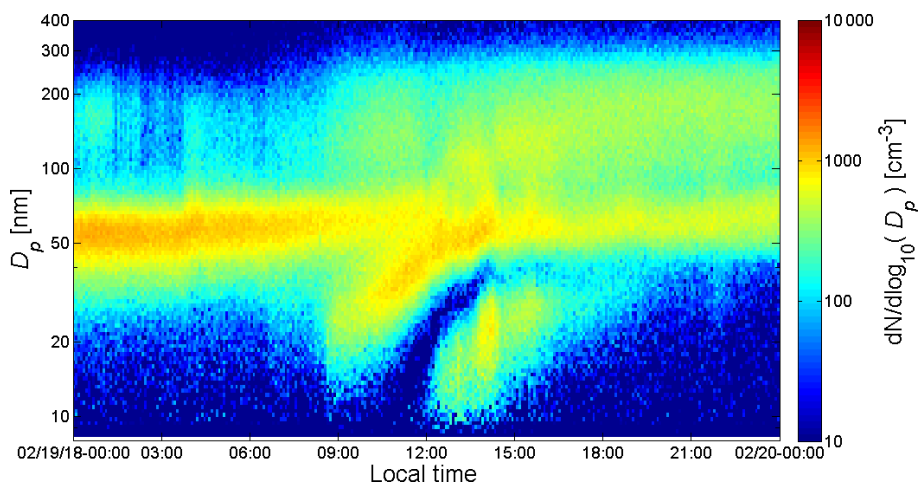
Figure 3. Characteristic examples of two CN_{<50} growth events at ATTO on 19 and 20 February 2018. The temporal evolution of the particle number size distribution (PNSD) is shown as a heat map, emphasizing the pronounced Aitken mode as well as particle growth events from the sub-50 nm particle to the Aitken mode during daylight.
