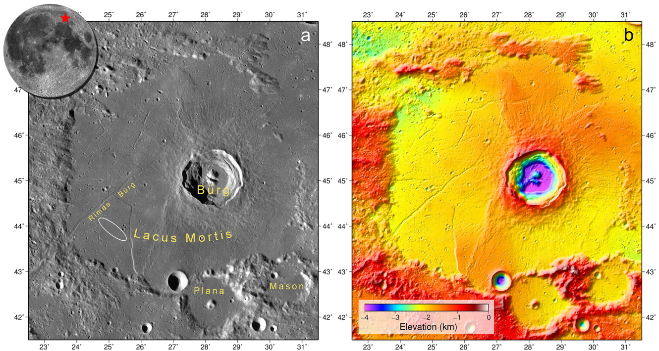
Figure 1. (a) A portion of the Lunar Reconnaissance Orbiter Camera (Robinson et al., 2010) Wide Angle Camera morphologic global mosaic with incidence angles between 55^\circ and 75^\circ (Speyerer et al., 2011; Wagner et al., 2015) showing the Lacus Mortis region in cylindrical equidistant projection with a standard parallel of 45^\circ\text{N} . White ellipse is the location of Astrobotic's Mission One landing ellipse. Inset nearside globe with red star marks the location of Lacus Mortis. (b) Shaded relief of the Lacus Mortis region colored by elevation (SLDEM2015) (Barker et al., 2016).
