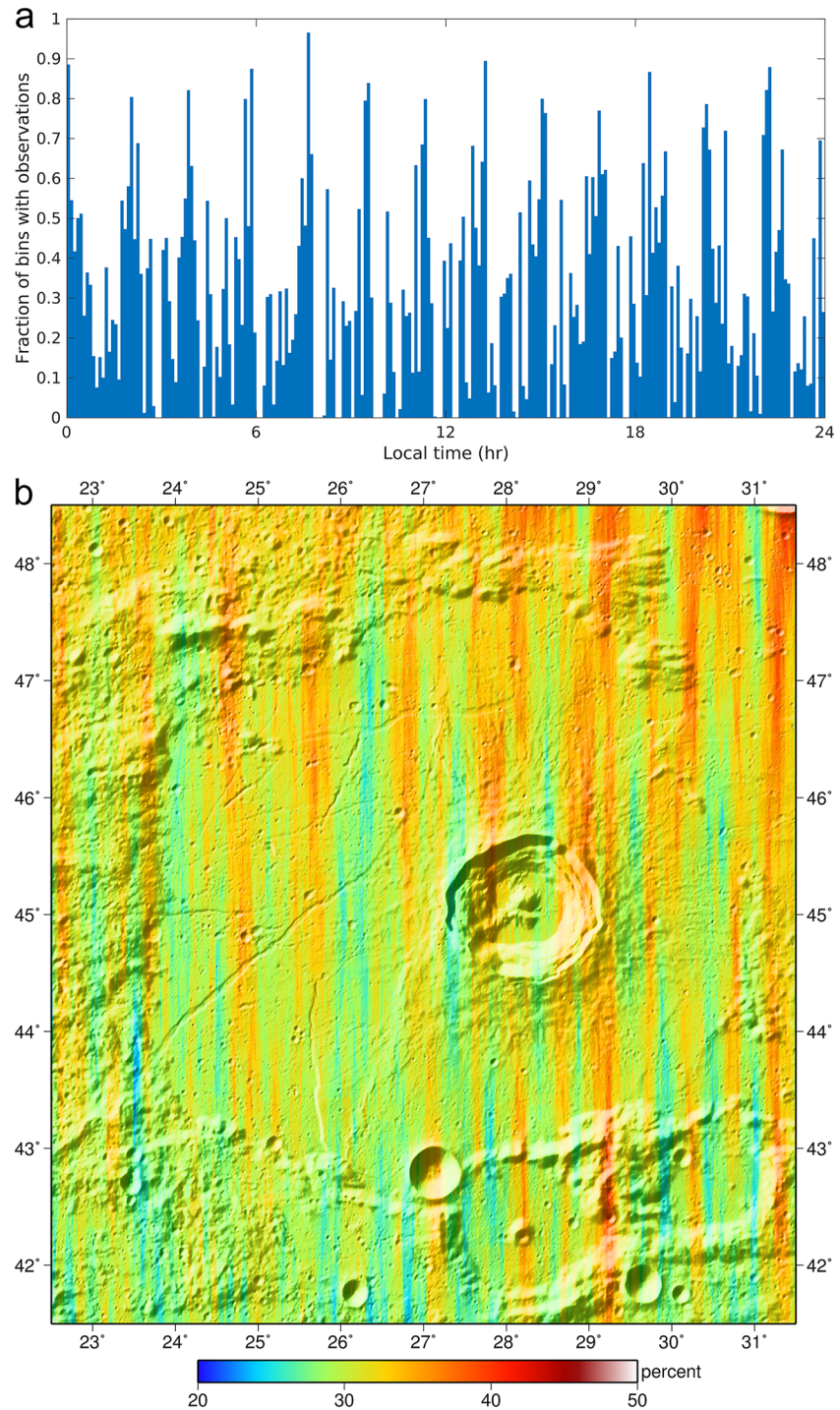
Figure 2. (a) A histogram of the 240 local time bins for the Lacus Mortis regions. (b) A map of the local time percent coverage (percentage of local time bins with data) of the region.
