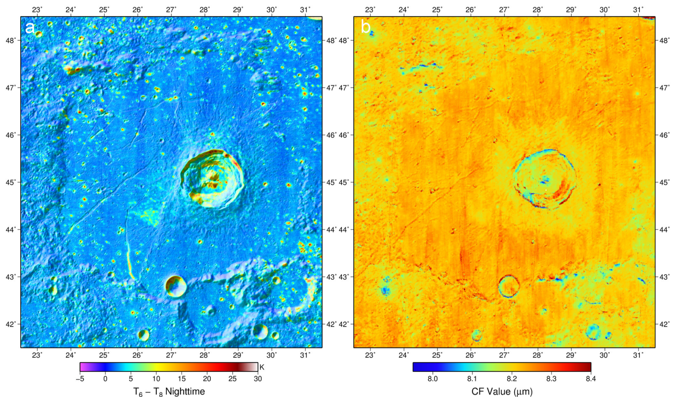
Figure 4. (a) Difference in nighttime temperatures between channels 6 and 8 ( T_6 - T_8 ) highlighting variations in anisothermality in Lacus Mortis. (b) Christiansen Feature value normalized to equatorial noon derived from Diviner channels 3 to 5.
