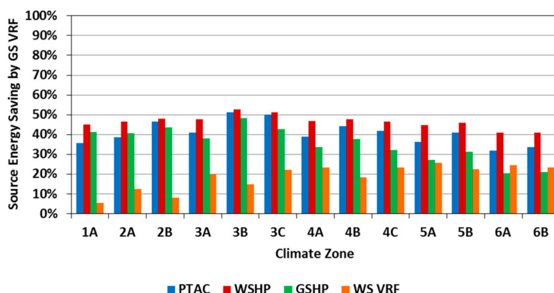
Figure 19. Source heating, ventilating, and air-conditioning (HVAC) energy savings of ground-source variable refrigerant flow (GS-VRF) systems compared to other HVAC systems for baseline office-building models in various U.S. climate zones.
