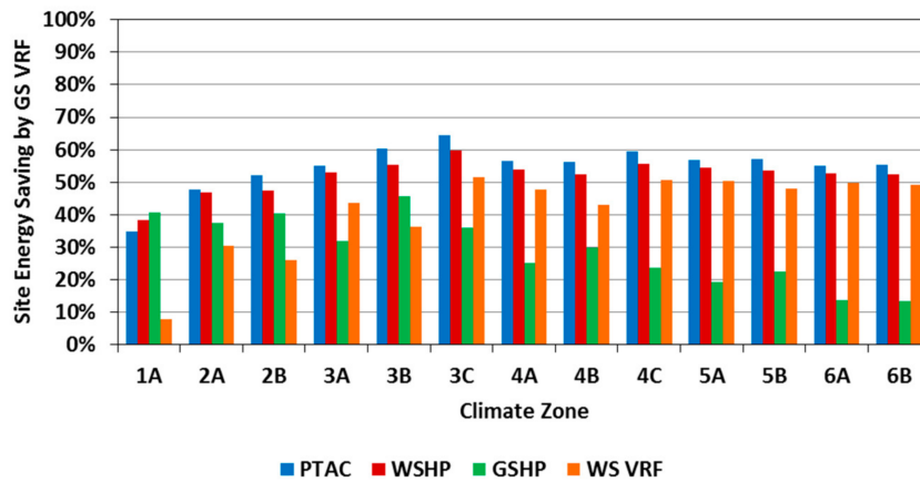
Figure 24. Site energy savings achieved by ground-source variable refrigerant flow (GS-VRF) systems compared to other HVAC systems for high-performance office buildings in various U.S. climates.
