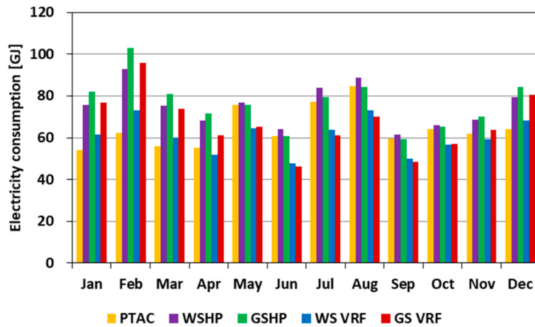
Figure 13. Monthly electricity consumption of various heating, ventilating, and air-conditioning (HVAC) systems for the office building located in Barberton, OH.
