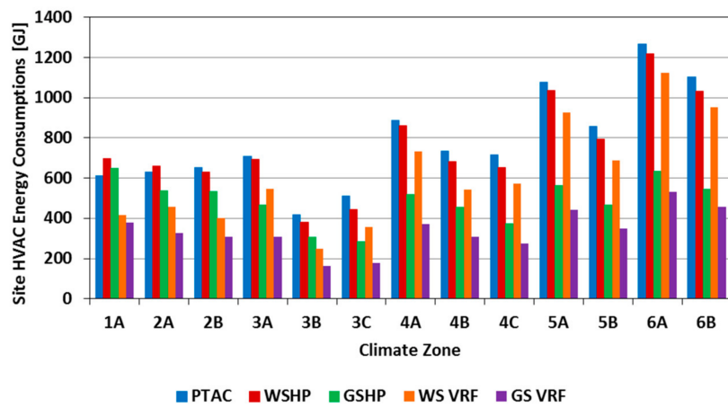
Figure 16. Site heating, ventilating, and air-conditioning (HVAC) energy use for baseline office-building models in various U.S. climate zones.
