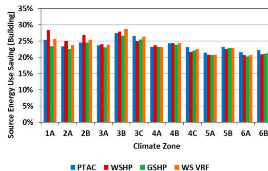
Figure 21. Source energy-use savings achieved by the high-performance designs compared to the baseline designs for office buildings located in various U.S. climates.
