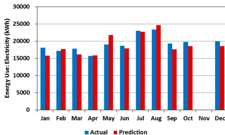
Figure 8. Calibration results of electricity use for the office-building energy model.
