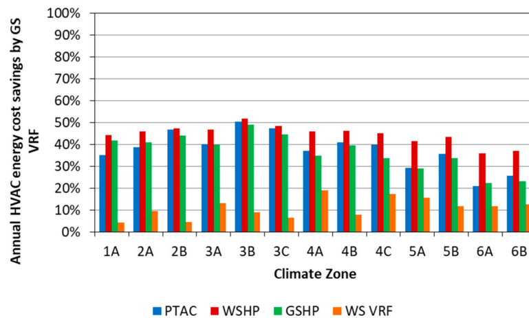
Figure 20. Annual heating, ventilating, and air-conditioning (HVAC) energy-cost savings achieved by ground-source variable refrigerant flow (GS-VRF) systems compared to other HVAC systems for the baseline building-office models in various U.S. climate zones.
