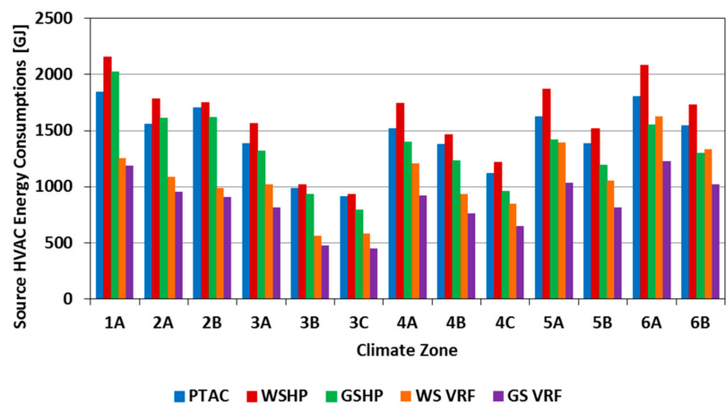
Figure 17. Source heating, ventilating, and air-conditioning (HVAC) energy use for baseline office-building models in various U.S. climate zones.
