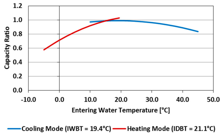
Figure 12. Capacity curves of a water-source variable refrigerant flow (VRF) system as a function of condensing medium temperature for both heating and cooling modes.
