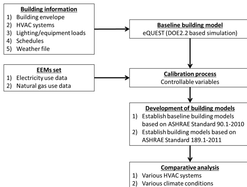
Figure 3. Flowchart for the simulation environment for the ground-source variable refrigerant flow (GS-VRF) evaluation analysis.
