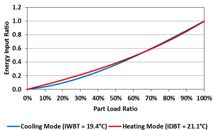
Figure 10. Part-load performance curves of a water-source variable refrigerant flow (VRF) system for both heating and cooling modes.
