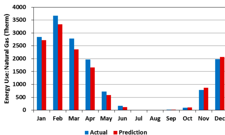
Figure 9. Calibration results of natural gas consumption for the office-building energy model.
