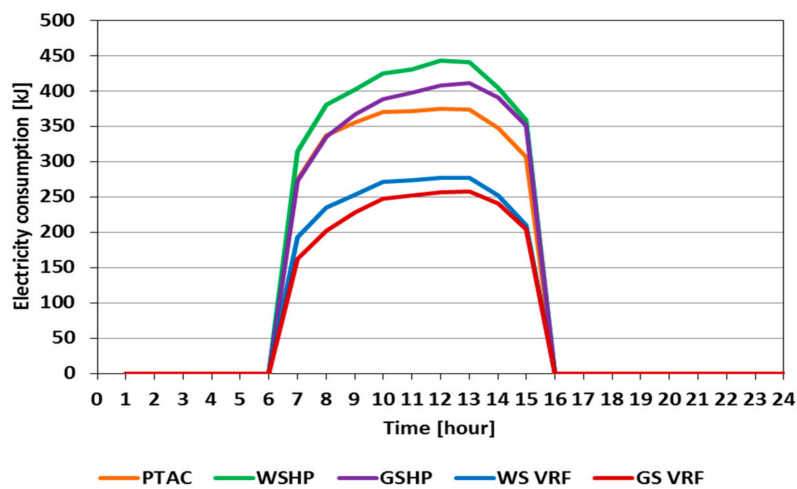
Figure 15. Hourly electricity use for various heating, ventilating, and air-conditioning (HVAC) systems during the cooling design day (July 21) for the office building in Barberton, OH.
