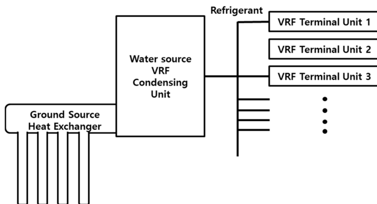
Figure 2. Typical components of ground-source variable refrigerant flow (VRF) system.
