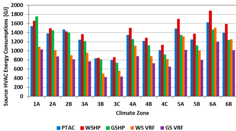
Figure 23. Source heating, ventilating, and air-conditioning (HVAC) energy use for high-performance office buildings in various U.S. climates.
