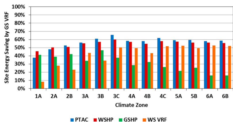
Figure 18. Site heating, ventilating, and air-conditioning (HVAC) energy savings of ground-source variable refrigerant flow (GS-VRF) systems compared to other HVAC systems for baseline office-building models in various U.S. climate zones.
