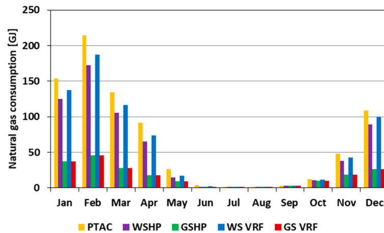
Figure 14. Monthly natural gas consumption of various heating, ventilating, and air-conditioning (HVAC) systems for the office building in Barberton, OH.
