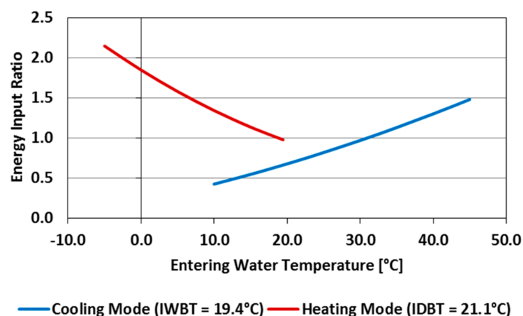
Figure 11. Energy efficiency curves of a water-source variable refrigerant flow (VRF) system as a function of condensing medium temperature for both heating and cooling modes.
