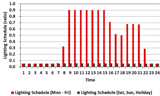
Figure 6. Lighting schedules used for the office-building model.
