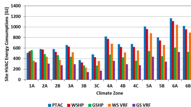
Figure 22. Site heating, ventilating, and air-conditioning (HVAC) energy use for high-performance office buildings in various U.S. climates.
