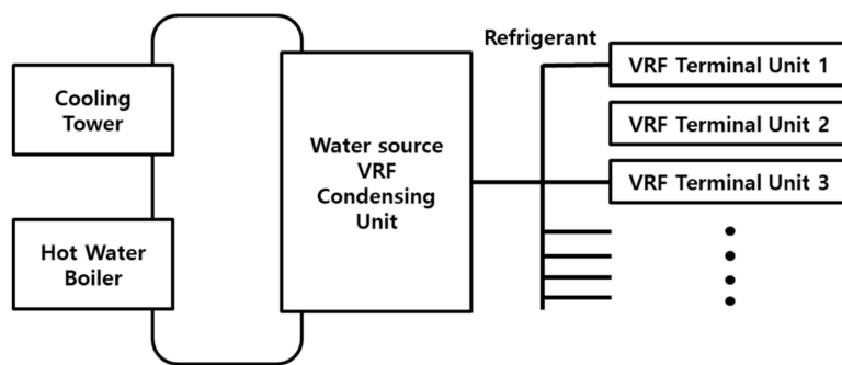
Figure 1. Typical components of a water-source variable refrigerant flow (VRF) system.
