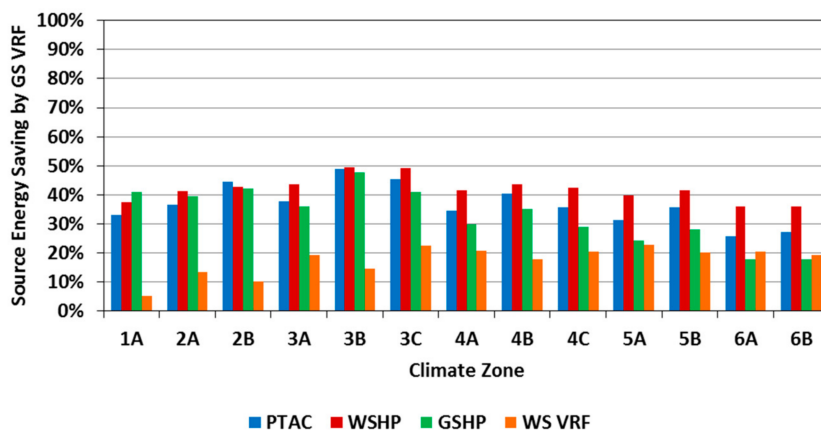
Figure 25. Source energy savings achieved by ground-source variable refrigerant flow (GS-VRF) systems compared to other heating, ventilating, and air-conditioning (HVAC) systems for high-performance office buildings in various U.S. climates.
