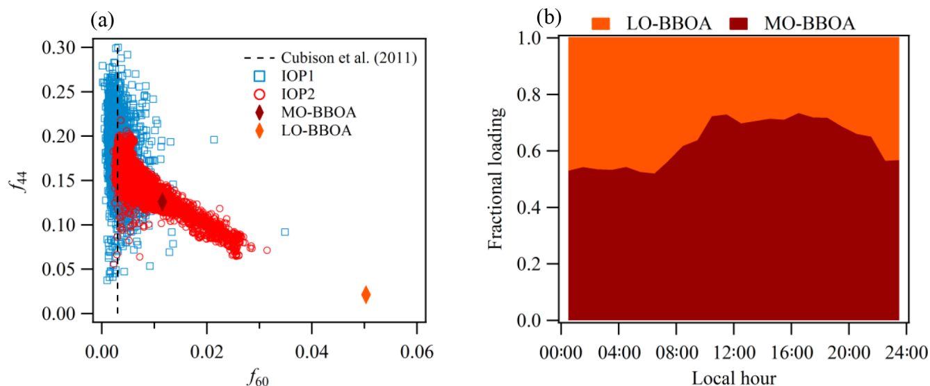
Figure 7. Analysis of the organic PM_{10} sampled at the T3 site in relation to biomass burning. (a) Scatter plot of the AMS signal fraction at m/z 44 ( f_{44} ) against that at m/z 60 ( f_{60} ). Red circles represent measurements during the dry season (IOP2), and blue squares represent measurements at the same site during the wet season (IOP1) (de Sá et al., 2018). Diamonds represent the MO-BBOA and LO-BBOA factors of IOP2. The dashed line represents a reference for negligible influence by biomass burning based on several field studies (Cubison et al., 2011). (b) Diel trends of the fractional loadings of the MO-BBOA and LO-BBOA factors relative to their sum BBOA_T . Local time is UTC minus 4 h.
