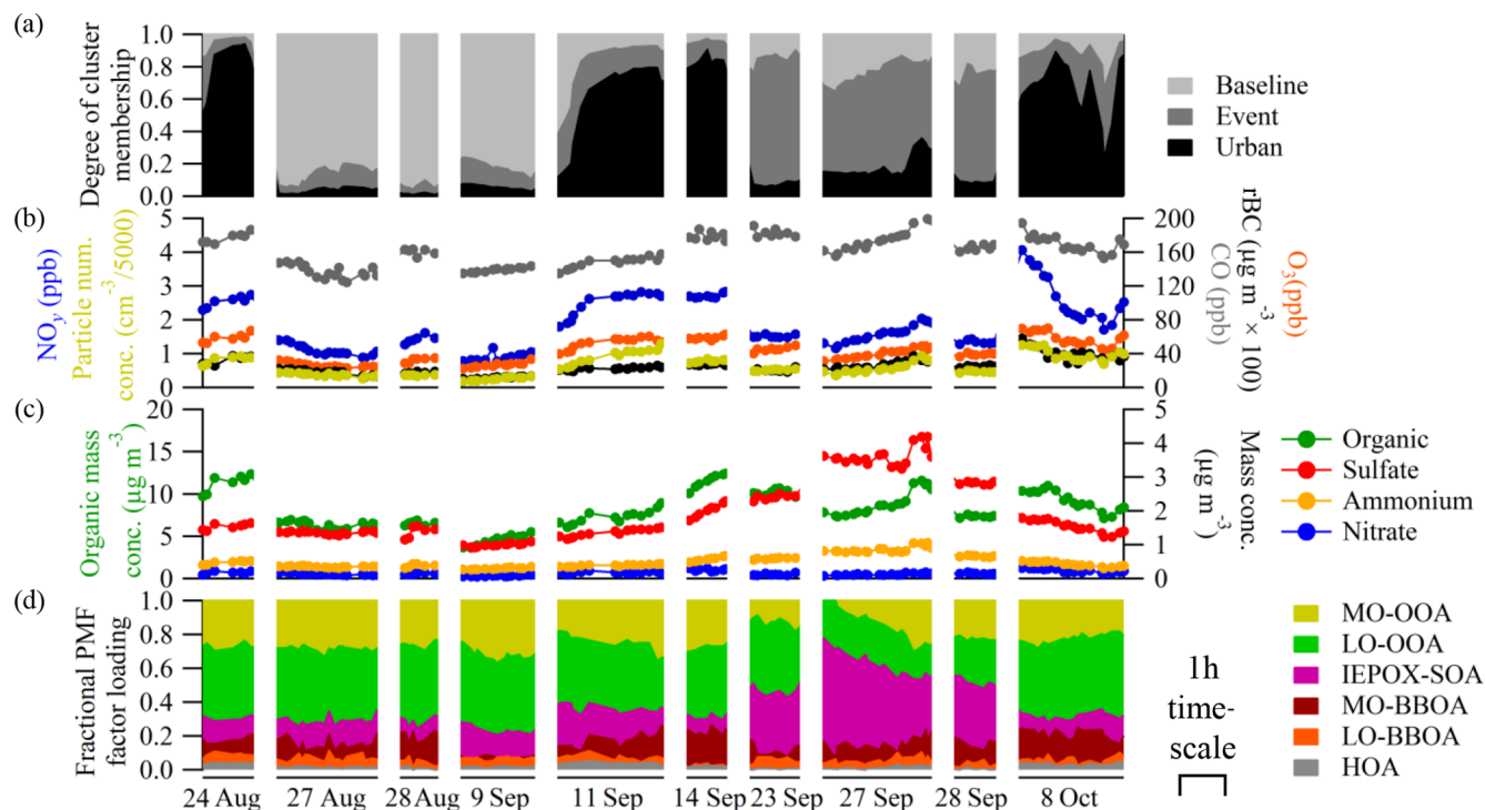
Figure 8. Results of the cluster analysis by FCM clustering for afternoon periods (12:00 to 16:00LT) presented by several case studies. The shown case studies represent 30 % of the FCM results. (a) Degree of membership in each of the three clusters. The sum of degrees of membership across all clusters is unity. (b) Pollution indicators: concentrations of \text{NO}_y , \text{O}_3 , CO, rBC, and particle number count are plotted. (c) \text{PM}_{10} mass concentrations for organic, sulfate, nitrate, and ammonium species. (d) Fractional contribution of each factor to the \text{PM}_{10} organic mass concentration.
