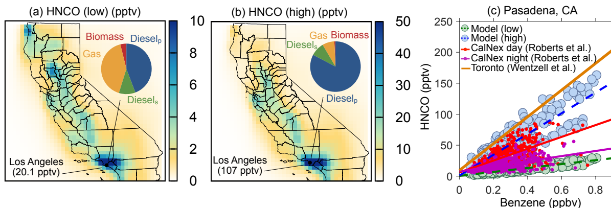
Figure 4. (a) Low and (b) high estimates of the 14-day averaged ground-level concentrations of HNCO from the 24 km simulations. The low and high estimates used two different primary emissions and photochemical production parameterizations for diesel engines (see Table 1). The color scales in panels (a) and (b) have been truncated at 10 and 50 pptv, respectively, to visualize the statewide variability in HNCO concentrations. We note that in both the panels, the HNCO concentrations in the Los Angeles region exceed the concentrations captured on the color scale. (c) 14-day averaged concentrations of HNCO regressed against benzene over the South Coast Air Basin from the 8 km simulations; also includes observations from Wentzell et al. (2013) for Toronto, 2012, and from Roberts et al. (2014) and Borbon et al. (2013) for Pasadena, 2010, during CalNex.
