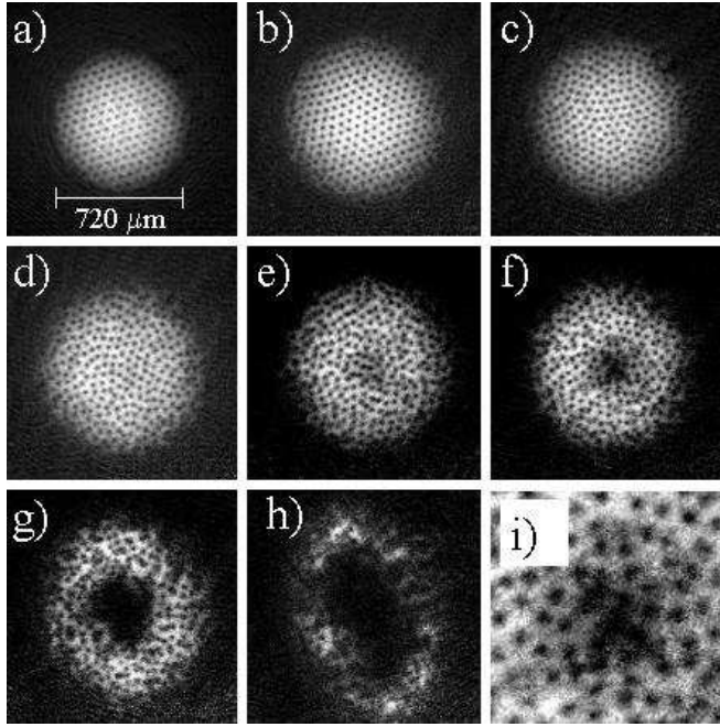
FIG. 1. Different stages of giant vortex formation process. (a) Starting point: BEC after evaporative spin-up. (b)-(h) Laser shone onto BEC for (b) 14 s, (c) 15 s, (d) 20 s, (e) 22 s, (f) 23 s, (g) 40 s, (h) 70 s. Pictures are taken after 5.7-fold expansion of the BEC. Laser power is 8 fW. (i) Zoomed-in core region of (f).
