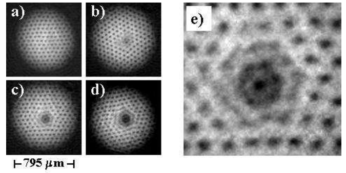
FIG. 3. Core developing after a 5 ms short, 2.5 pW laser pulse. In-trap evolution time after end of pulse is (a) 0.5 ms, (b) 10.5 ms, (c) 20.5 ms, (d) 30.5 ms. Images taken after sixfold expansion of BEC. (e) Zoomed-in core region of (c).
