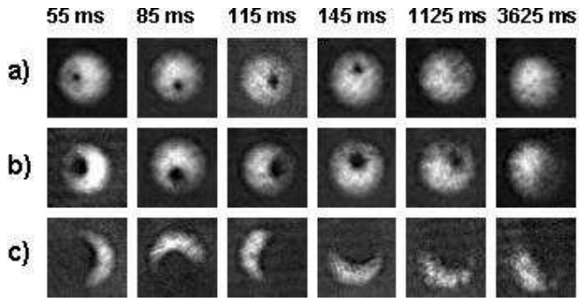
FIG. 5. Giant core precession. Cores created by a 10 ms off-centered laser pulse with a power of (a) 4.2 pW, (b) 33 pW, (c) 470 pW. Time given in figure is in-trap evolution time after end of laser pulse. For reference, a naive expectation for the lifetime of a giant vortex given by the radius of the core divided by the speed of sound in the surrounding cloud would be 13 ms and 30 ms for (a) and (b), respectively.
