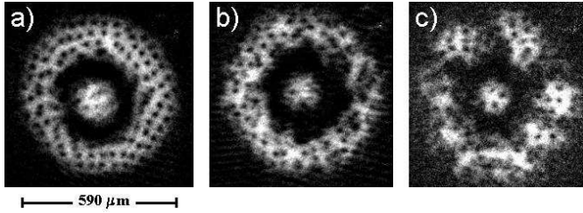
FIG. 6. Ring cut out of a BEC by a 125 ms long, off-centered laser pulse. Expansion image taken (a) directly after end of pulse (b) after an additional in-trap evolution time of 200 ms after end of pulse and (c) evolution time 2 s.
