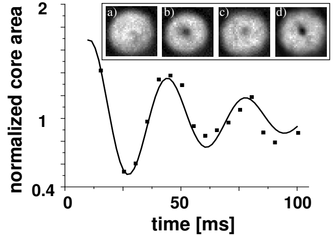
FIG. 4. Oscillation of core area after an 8 pW, 5 ms laser pulse. Starting conditions are 2.5 \times 10^6 atoms with rotation rate 0.9 \omega_p . Time given is in-trap evolution time after end of pulse. Core area is normalized to mean of all data points. Inset: Initial conditions 3.5 \times 10^6 atoms with rotation rate 0.78 \omega_p ; in-trap images taken after a 14 pW, 5 ms laser pulse followed by evolution time of (a) 20 ms, (b) 40 ms, (c) 60 ms, and (d) 80 ms.
