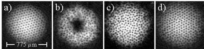
FIG. 2. Lattice reforming after giant vortex formation. (a) BEC after evaporative spin-up. (b) Effect of a 60 fW, 2.5 s laser pulse. (c),(d) Same as (b), but additional 10 s (c) and 20 s (d) in-trap evolution time after end of laser pulse. Images taken after a sixfold expansion of the BEC.
