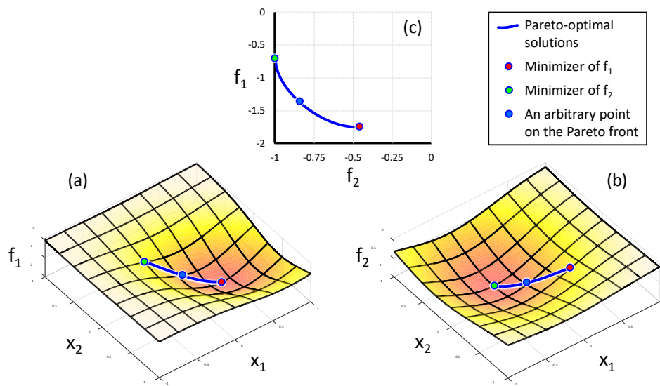
Figure 5. Illustration of the relationship between (a) the fitness landscape of objective 1, (b) the fitness landscape of objective 2 and (c) the Pareto-front of the two-objective optimization problem.
