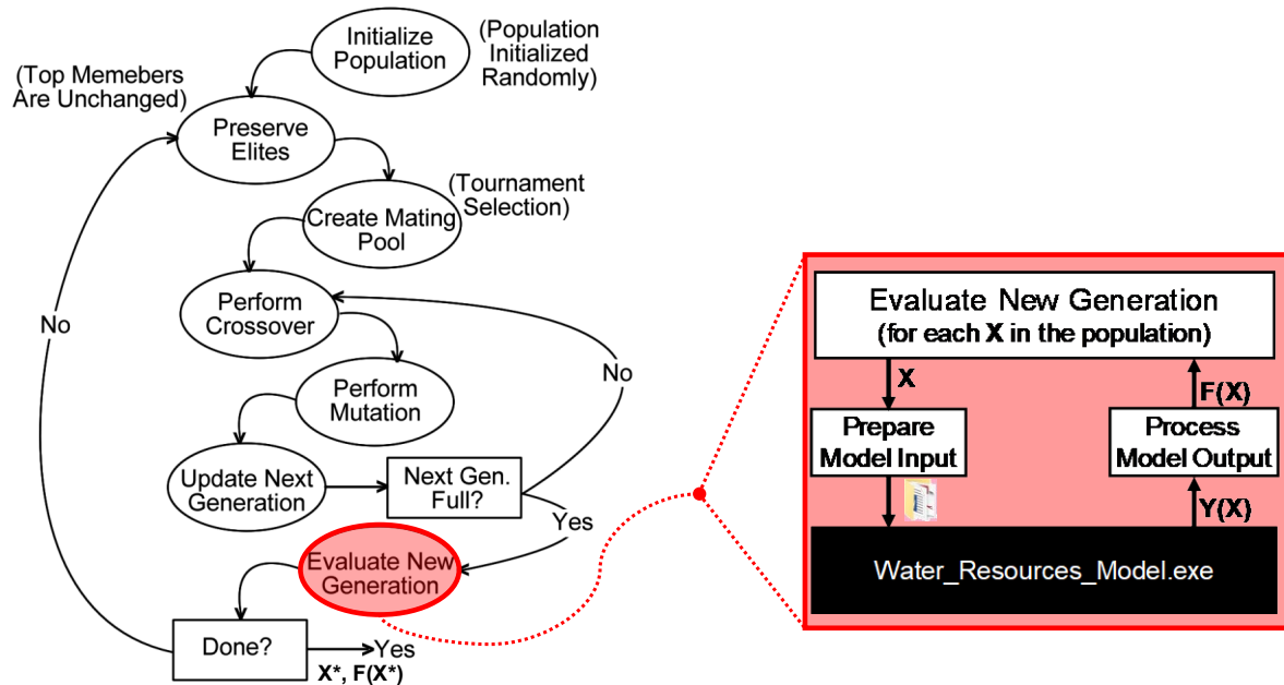
Figure 17. Illustration of the 'black-box' approach to linking an evolutionary algorithm with a water resources model. \mathbf{x} and f(\mathbf{x}) are as described in equations 1-3 (see Section 3.1) and \mathbf{y}(\mathbf{x}) represents a set of model outputs (response variables) that are computed as a function of the decision variables (i.e. \mathbf{x} ) represents a vector of objective functions and/or constraints that are to be optimized and which are computed using the model outputs.
