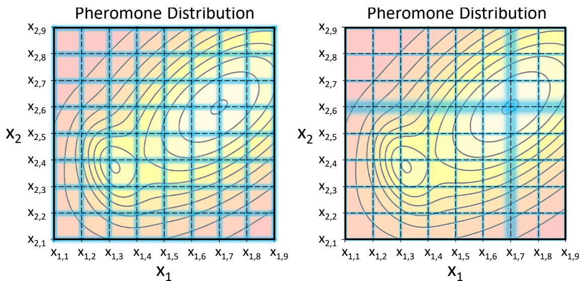
Figure 13. Illustration of the evolution of pheromone concentrations over a large number of iterations, where the thickness of the blue shading of the paths corresponding to discrete decision variable choices corresponds to pheromone concentration. As can be seen, the discrete values of X_1 and X_2 that correspond to the globally optimal solution (i.e. X_{1,7} and X_{2,6} ) have higher pheromone concentrations during the final iteration, thereby increasing the probability that these decision variable values will be selected.
