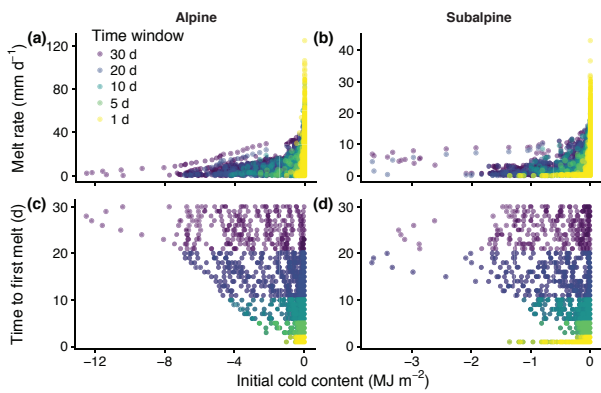
Figure 11. Simulated sub-seasonal snowmelt rate plotted against initial cold content in the alpine (a) and subalpine (b), and time to first melt plotted against initial cold content in the alpine (c) and subalpine (d) for time windows from 1 to 30 days.
