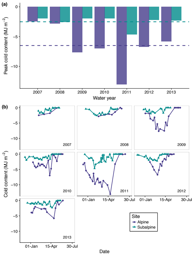
Figure 2. Peak annual cold content (a) and individual snow pit observations of cold content (b) for the alpine and subalpine from WY2007–WY2013. The dashed horizontal lines in (a) represent the mean peak annual cold content values for the two sites.
