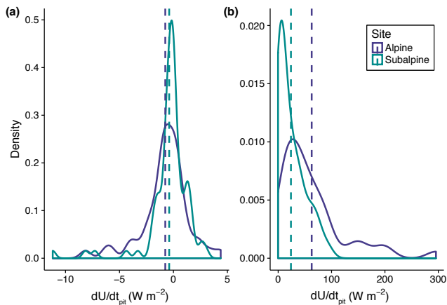
Figure 4. Kernel density estimates of \frac{dU}{dr_{\text{pit}}} distributions as calculated from snow pit observations for periods with SWE gain (a) and loss (b) in the alpine and subalpine for WY2007–WY2013. The dashed vertical lines represent the mean \frac{dU}{dr_{\text{pit}}} for the alpine (a: -0.8 \text{ W m}^{-2} ; b: 62.8 \text{ W m}^{-2} ) and subalpine (a: -0.4 \text{ W m}^{-2} ; b: 23.9 \text{ W m}^{-2} ).
