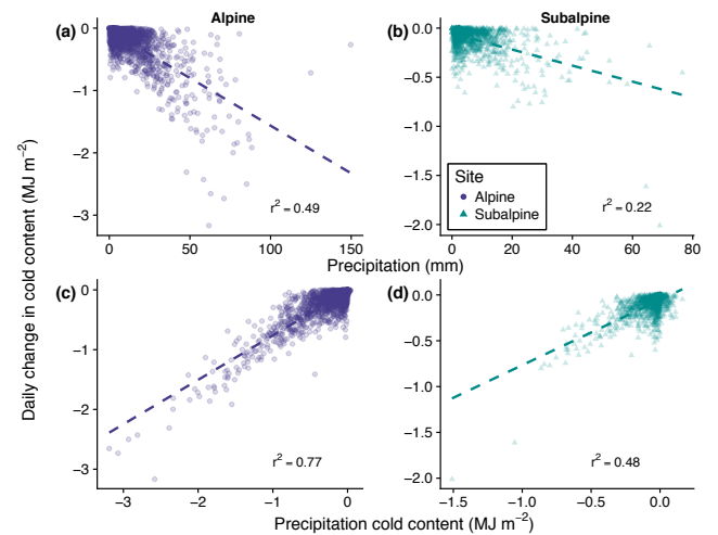
Figure 9. Simulated daily change in cold content plotted against daily precipitation in the alpine (a) and subalpine (b), and cold content from precipitation in the alpine (c) and subalpine (d).
