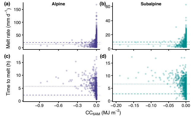
Figure 12. Simulated daily melt rates in the alpine (a) and subalpine (b) and time to snowmelt in the alpine (c) and subalpine (d) as a function of CC_{06:00AM} . The dashed line in each figure represents the mean melt rate (a, b) and time to melt (c, d) for days when CC_{06:00AM} = 0 \text{ MJ m}^{-2} and the dotted line represents those quantities for days when CC_{06:00AM} < 0 \text{ MJ m}^{-2} .
