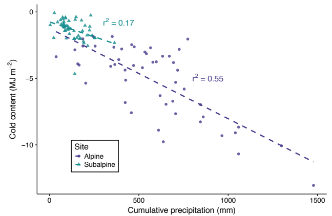
Figure 3. Cold content plotted against cumulative precipitation from 1 December to the date of snow pit observation for the alpine and subalpine for the snow season up to and including the date of peak cold content from WY2007 to WY2013. The dashed lines of best fit were calculated using ordinary least squares linear regression.
