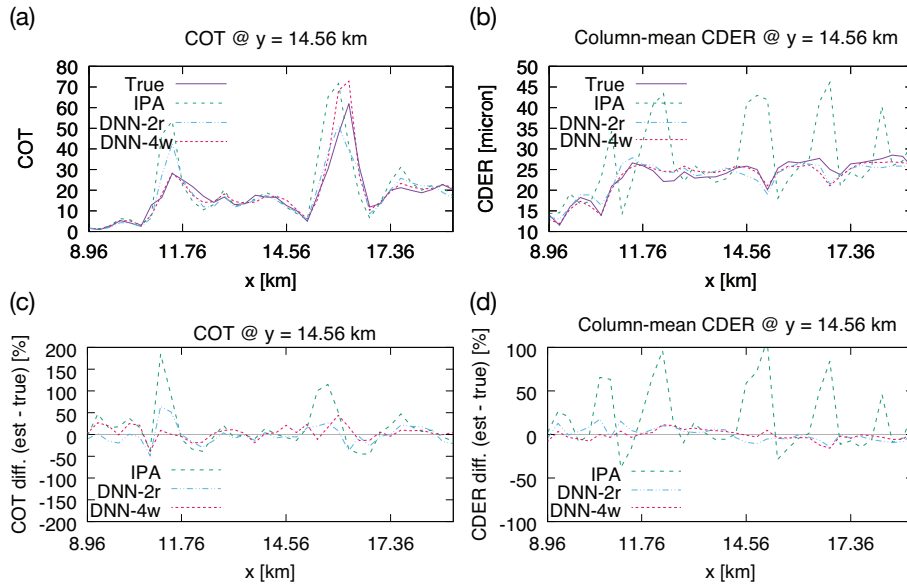
Figure 6. Examples of horizontal distribution of estimated (a) COT and (b) CDER by the IPA retrieval and DNNs for a view zenith angle of 0^\circ at y = 14.56 km in Fig. 5 and the relative error of the estimated (c) COT and (d) CDER. The sun is located on the left-hand side with an SZA of 60^\circ .
