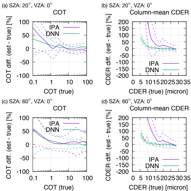
Figure 7. Comparison of retrieval errors of DNN-4w and IPA retrieval for SZAs of (a, b) 20^\circ and (c, d) 60^\circ . The horizontal axes show the true values of either COT or column-mean CDER. The vertical axes show the relative error of the estimated cloud property. The solid and dashed lines denote mean errors and means \pm standard deviations of error, respectively.
