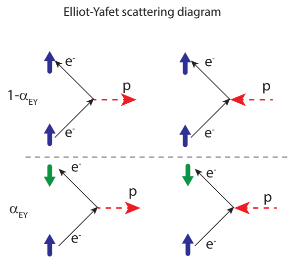
Figure 4.4: illustration of the Elliot-Yafet scattering mechanism. An electron flips its spin by creating or absorbing a phonon with \alpha_{\text{EY}} probability.
