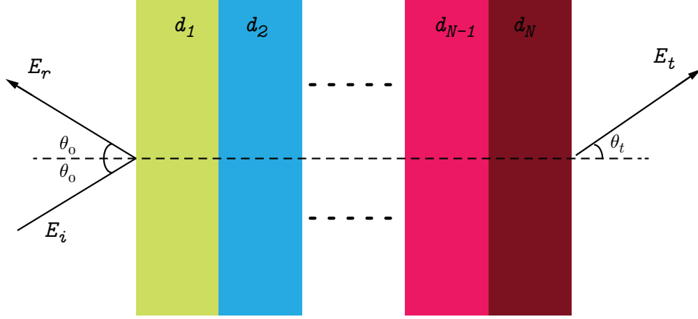
Figure 2.8: Illustration of multilayer structure. The experimental system I study is composed of N layers with the s substrate at the bottom. Each interface has a dynamics matrix, and each layer has a propagation matrix. The relationship of the transmitted and reflected electric fields can be found by multiplication of all the dynamics and propagation matrices.
