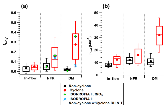
Figure 13. Statistical representation of the distribution of (a) aerosol nitrate fraction ( f_{\text{NO}_3} = \text{NO}_3^- / [\text{NO}_3^- + \text{HNO}_3] ) and (b) aerosol optical extinction within the three studied regions during non-cyclone and cyclone periods. The box and whiskers indicate 10th, 25th, 75th, and 90th percentiles, while the solid lines and circles mark the median and mean values, respectively. Modeled f_{\text{NO}_3} values with actual inputs of chemical composition and T and RH are shown with green diamonds, while the predicted values with the non-cyclone composition and cyclone T and RH are shown with blue stars.
