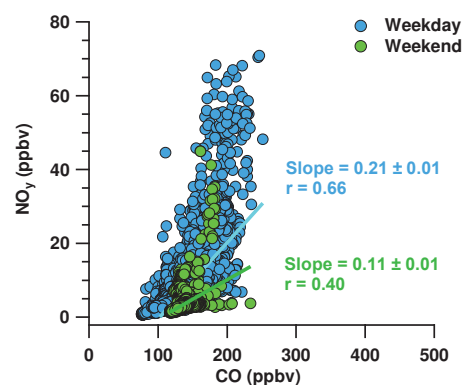
Figure 11. Scatterplot of measured \text{NO}_y vs. \text{CO} using aircraft data from the DISCOVER-AQ P-3 flights. Weekday (blue dots, 8 combined days) and weekend (green dots, 4 combined days). Inferred slopes are derived from ODR error-weighted (5% \text{NO}_y , 2% \text{CO} ) fits.
