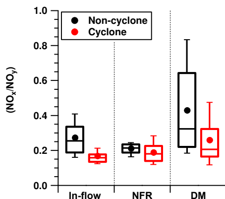
Figure 10. Statistical representation of the distribution of the mixing ratios of \text{NO}_x/\text{NO}_y within the three study regions. The box and whiskers indicate 10th, 25th, 75th, and 90th percentiles, while the solid lines and circles mark the median and mean values, respectively.
