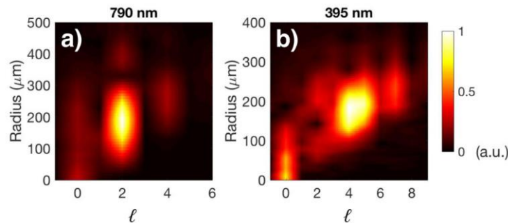
Fig. 3. Retrieved OAM spectrum of the two reconstructed vortex beam fields obtained by Fourier transformation of the fields along the azimuthal direction for different radii, for (a) 790 nm and (b) 395 nm. The color map corresponds to the spectrum in arbitrary units (a.u.). Note that the resolution in the OAM number \ell is limited to one from Fourier transform of the azimuthal coordinate; the plot has been interpolated for smoothness. In addition, the Fourier transform is in the range \ell = \pm 60 , but here we present the section of the spectrum with the highest yield. High yield is seen at \ell = 2 for \lambda = 790 nm and at \ell = 4 for \lambda = 395 nm as expected.
