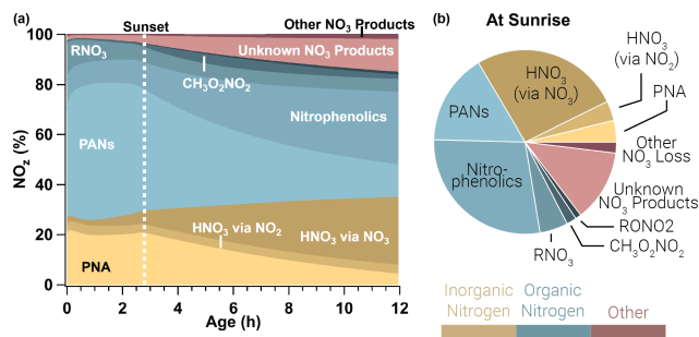
Figure 10. Relative integrated \text{NO}_x reservoirs and sinks for the WF2 model run as a function of plume age (a) and at sunrise (b). This result is the average between a WF2 model run constrained and unconstrained to peroxyacetyl nitrate observations as explained in the main text. Gold colors indicate inorganic nitrogen, blue colors indicate organic nitrogen, and red colors indicate other forms of \text{NO}_z . In this analysis we consider HONO to be a member of \text{NO}_x rather than \text{NO}_z . PANs and PNA dominate \text{NO}_z during the daytime, but after sunset these decompose to provide \text{NO}_2 that is subsequently lost to nitrophenolics and other \text{NO}_3 products overnight.
