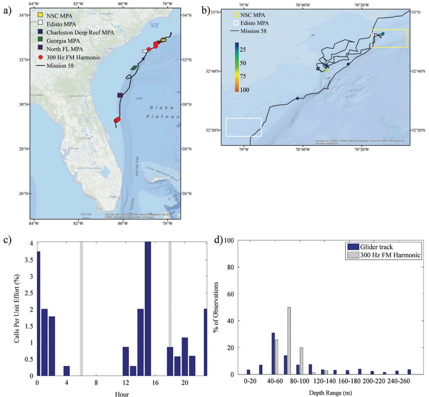
FIGURE 6. (a) Locations of acoustic files that contained 300-Hz FM harmonic sounds across the entire glider track (red circles; N = 70 ); (b) locations of those same files zoomed in to the northern portion of the track and binned as a percentage of 30-s files per hour; (c) percentage of 30-s files containing 300-Hz FM harmonic sound production normalized by the total number of files that were recorded during each hour (gray bars indicate local sunrise and sunset); and (d) percentage of 300-Hz FM harmonic observations and the overall glider track present within 20-m bottom depth intervals. Site abbreviations used in panels (a) and (b) are defined in Figure 1.
