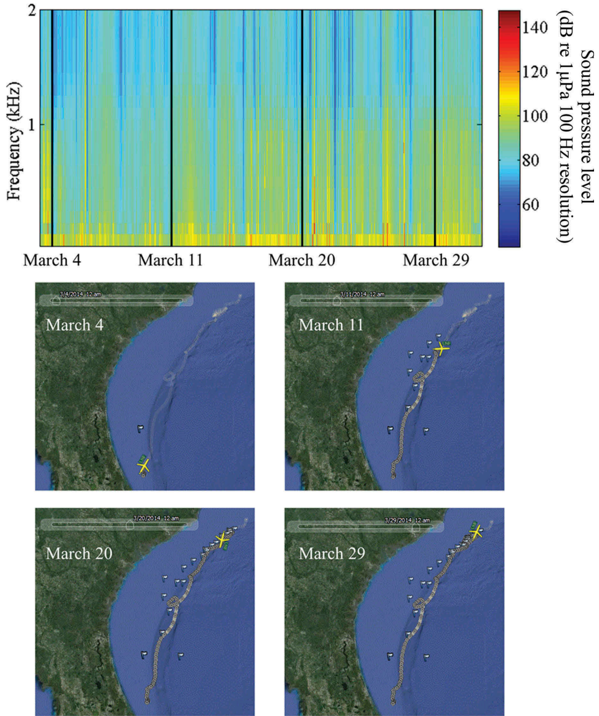
FIGURE 2. Composite spectrogram, showing the band sound pressure level (dB referenced to 1 \mu Pa; 100-Hz resolution) up to 2 kHz, with four date marks (all dates are from 2014; upper panel); and the corresponding position of the autonomous glider along the southeastern U.S. coast on those dates (lower panels). The yellow symbol in the lower panels represents the glider; the direction the icon is facing indicates the glider's heading. The white flags represent waypoints that were used to navigate the glider during the mission.
