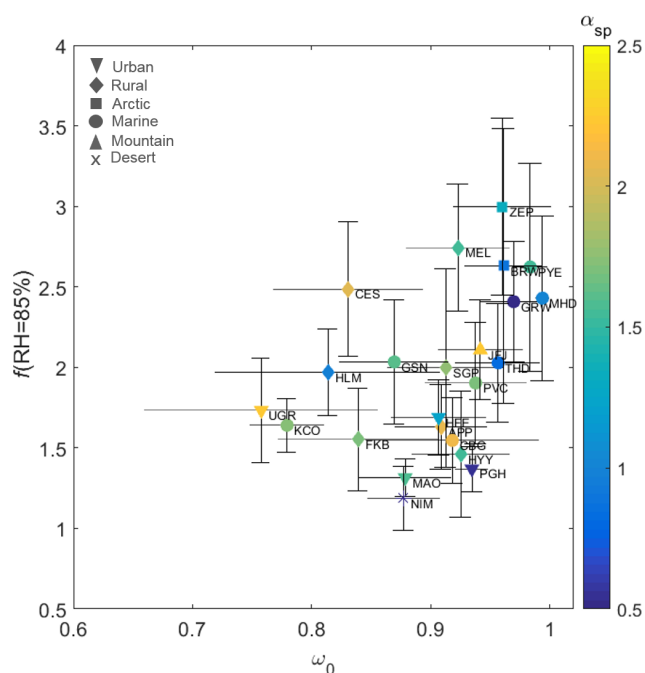
Figure 7. Scatterplot of mean f(\text{RH} = 85\%) versus single-scattering albedo, \omega_0 , at 550 nm ( \lambda = 525 nm at HYY) color-coded by the scattering Ångström exponent, \alpha_{sp} , for the wavelength pair 450–700 nm at each site. The dots represent the mean value, and the error bars are the standard deviation.
