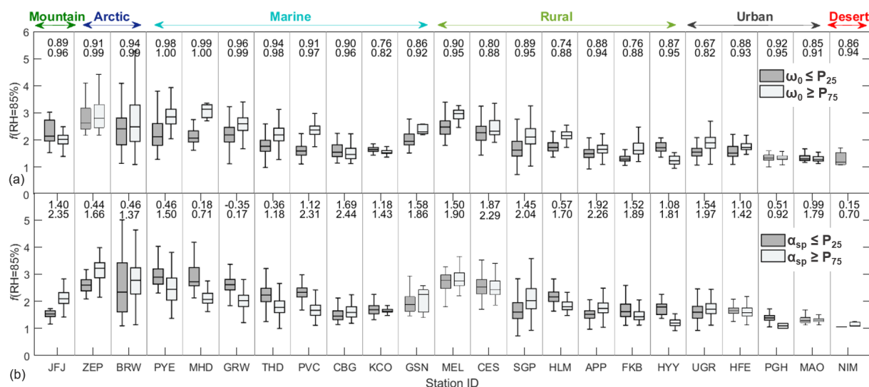
Figure 6. Box plot of f(\text{RH} = 85\%) at 550 nm ( \lambda = 525 nm at HYY) segregated by single-scattering albedo ( \omega_0 ) values (a) and scattering Ångström exponent ( \alpha_{sp} ) values (b). Sites are sorted by site type and decreasing f(\text{RH} = 85\%) . For each box, the central mark is the median, the box extends vertically between the 25th and 75th percentiles, and the whiskers extend to the most extreme data that are not considered outliers. The numbers on top indicate the 25th and 75th percentiles used for segregating each dataset. Categories that are not significantly different are shown with thinner lines in the box plot.
