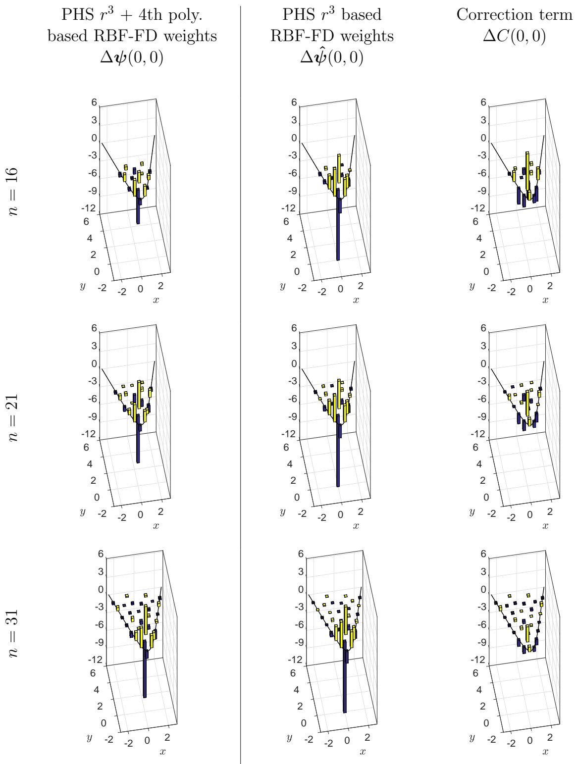
Figure 16: Same as Figure 14 but for the 2-D stencil (c) displayed in Figure 8.
