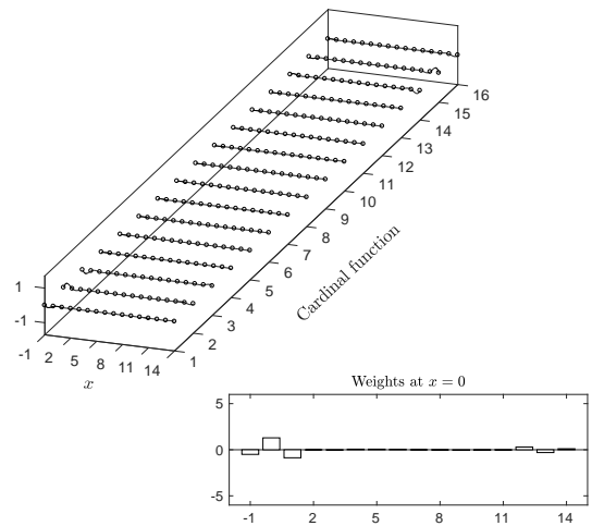
Figure 4: PHS+poly cardinal functions from Figure 1, split according to equation (9) into pure PHS cardinal functions \hat{\psi}(x) (left column) and correction term \underline{C}(x) (right column). The weights in the right column of the subplots, when added to the ones in the left column, leads to the RBF-FD weights displayed in Figure 1, ensuring the specified order of accuracy.
