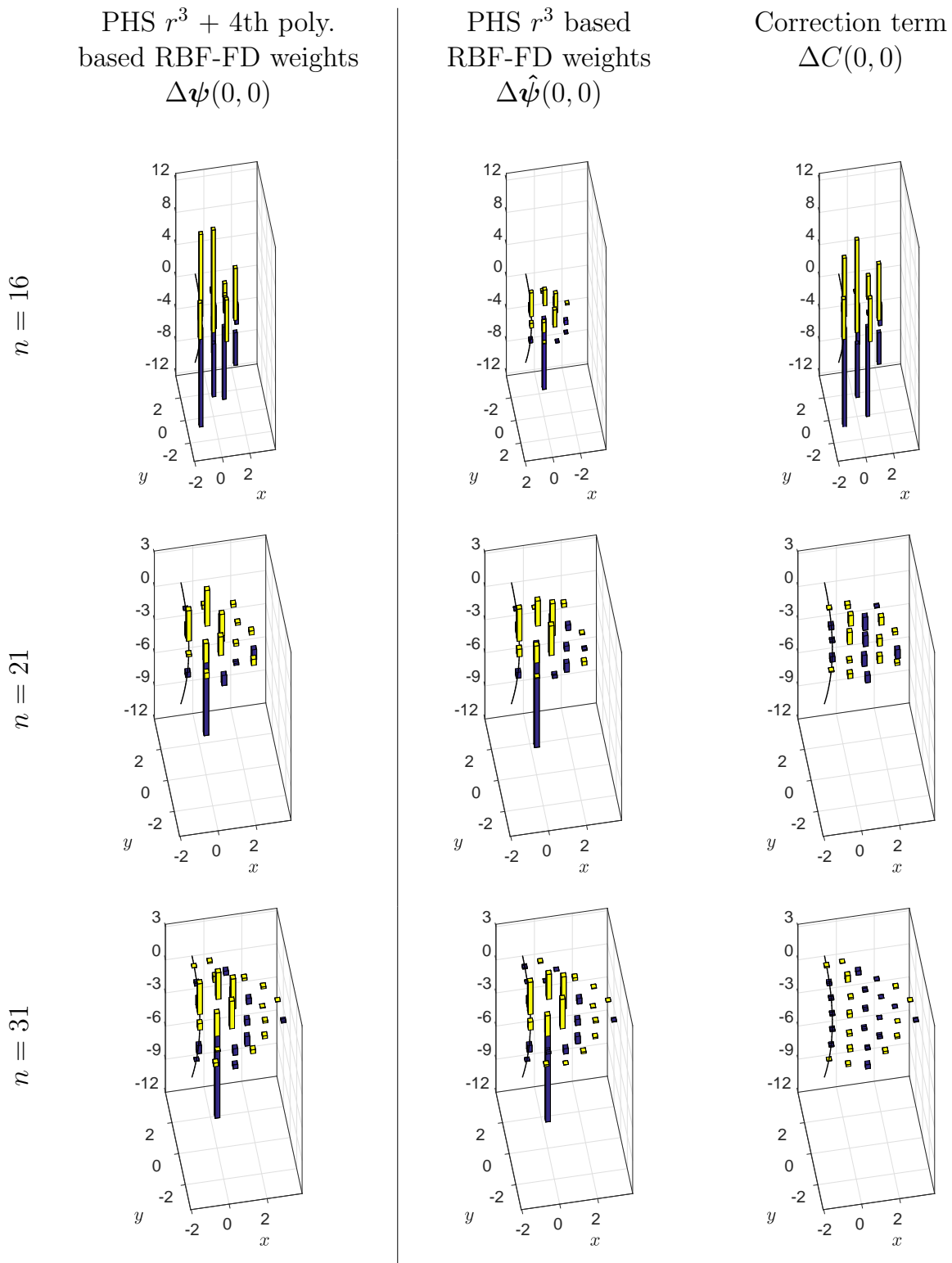
Figure 15: Same as Figure 14 but for the 2-D stencil (b) displayed in Figure 8.
