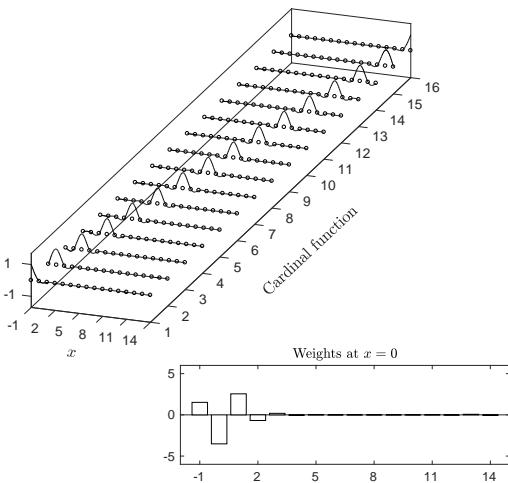
Figure 4: PHS+poly cardinal functions from Figure 1, split according to equation (9) into pure PHS cardinal functions \hat{\psi}(x) (left column) and correction term \underline{C}(x) (right column). The weights in the right column of the subplots, when added to the ones in the left column, leads to the RBF-FD weights displayed in Figure 1, ensuring the specified order of accuracy.
