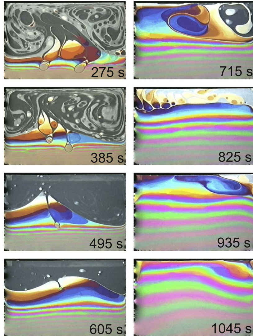
Figure 8. Climbing of smectic layers in a vertically suspended film under the influence of a vertical temperature gradient. A thermostated block at the lower frame edge was set to a temperature of T_h = 70^\circ\text{C} . The top of the frame was not heated. It remained approximately at room temperature ( 25^\circ\text{C} ). Images are 33 \times 20 \text{ mm}^2 . The smectic material is the commercial mixture FELIX16-100 (Hoechst). During the first 10 min, hot air flowing upwards induces a pair of convection rolls in the upper thin film region (thickness \approx 80 \text{ nm} ). The thicker regions that climb up are less sensitive to air flow, thus the convection ceases.
