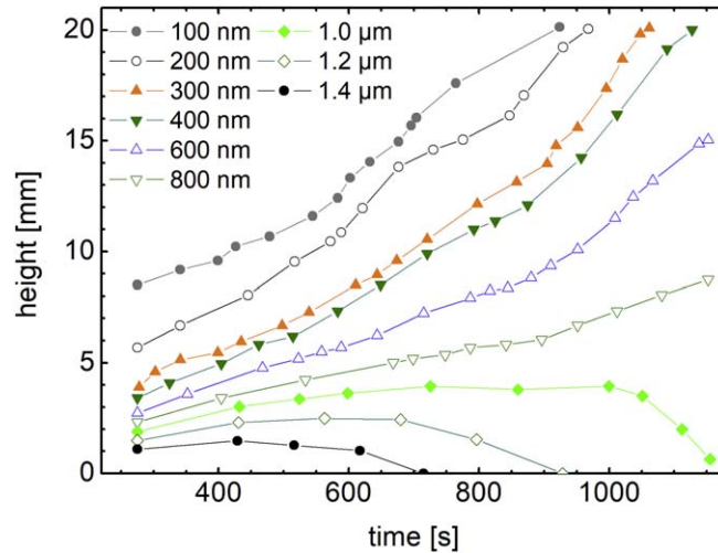
Figure 9. Climbing of smectic layers in the film shown in figure 8. Since the zones of equal thickness are not exactly horizontal but perturbed by convection, the heights represent averages over width of the film.
