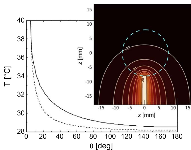
Figure 5. Calculated temperature profile at the smectic bubble surface established by heat conduction of the ambient air, with the supporting needle at 40 °C and the chamber walls at 28 °C. The solid curve represents the numerically computed profile. For comparison, the dashed curve shows the analytical result for a spherical heat source with radius r_c at the needle tip. The inset shows the stationary, axially symmetric solution of the heat diffusion equation, with contour lines in 2 K steps. The bubble is indicated by the dashed circle.
