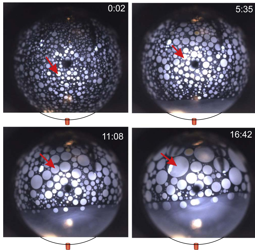
Figure 4. Islands on a smectic bubble migrating under the influence of a thermal gradient (needle at 40 °C, chamber walls at 28 °C). The material is a commercial smectic A mixture (see text). A selected island is marked by arrows to indicate the upward drift. The dark spot facing the observer is a technical artefact. The position of the heated needle tip is sketched below the images. The images were taken from a sequence recorded at a frame rate of 30 fps. Time is shown in the form min:s in each image.
